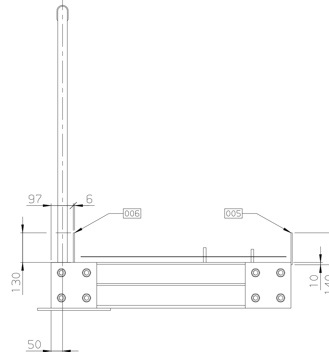
VIEW B
