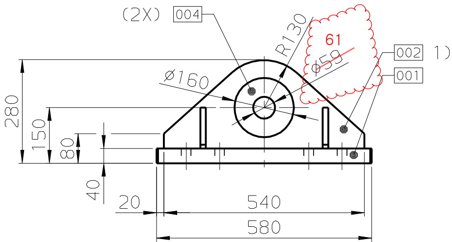
VIEW A
