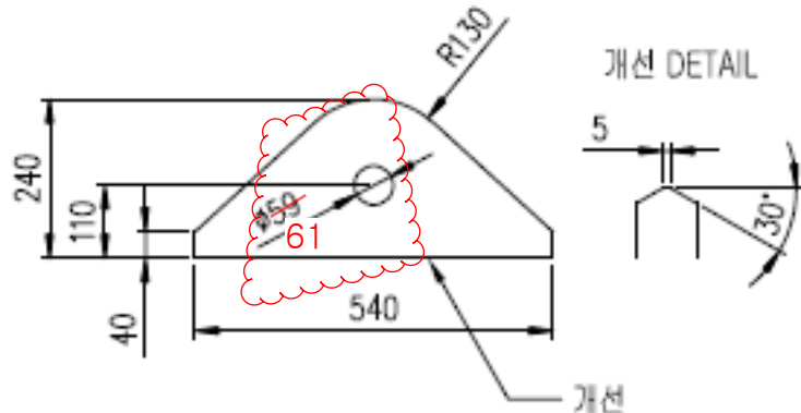
POS 002 THICKNESS 45mm
