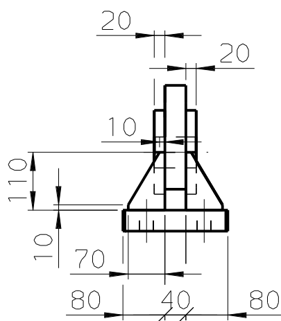
VIEW B
