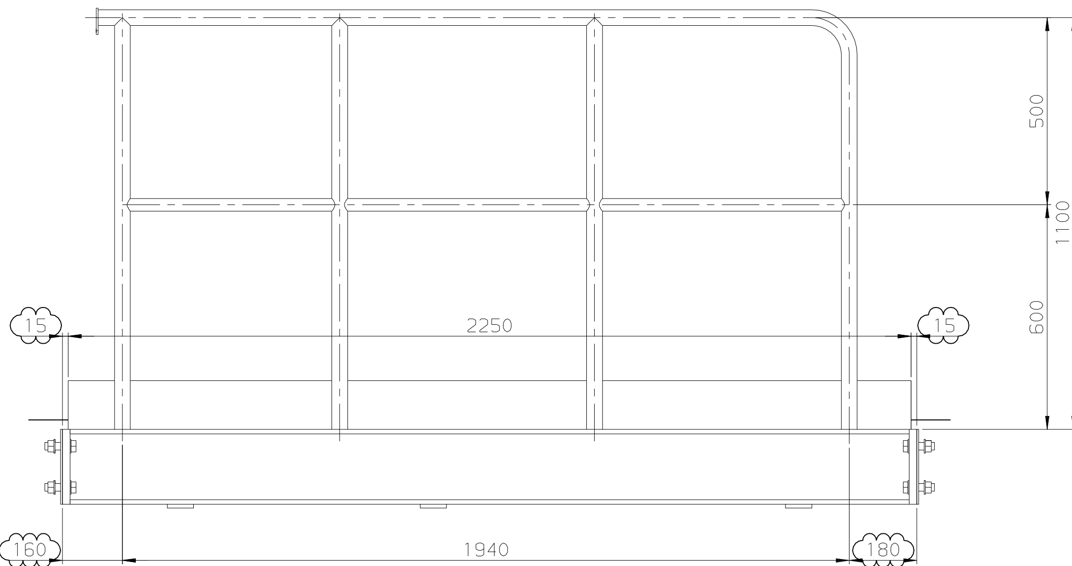
VIEW C
