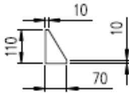
POS 003 THICKNESS 15mm
