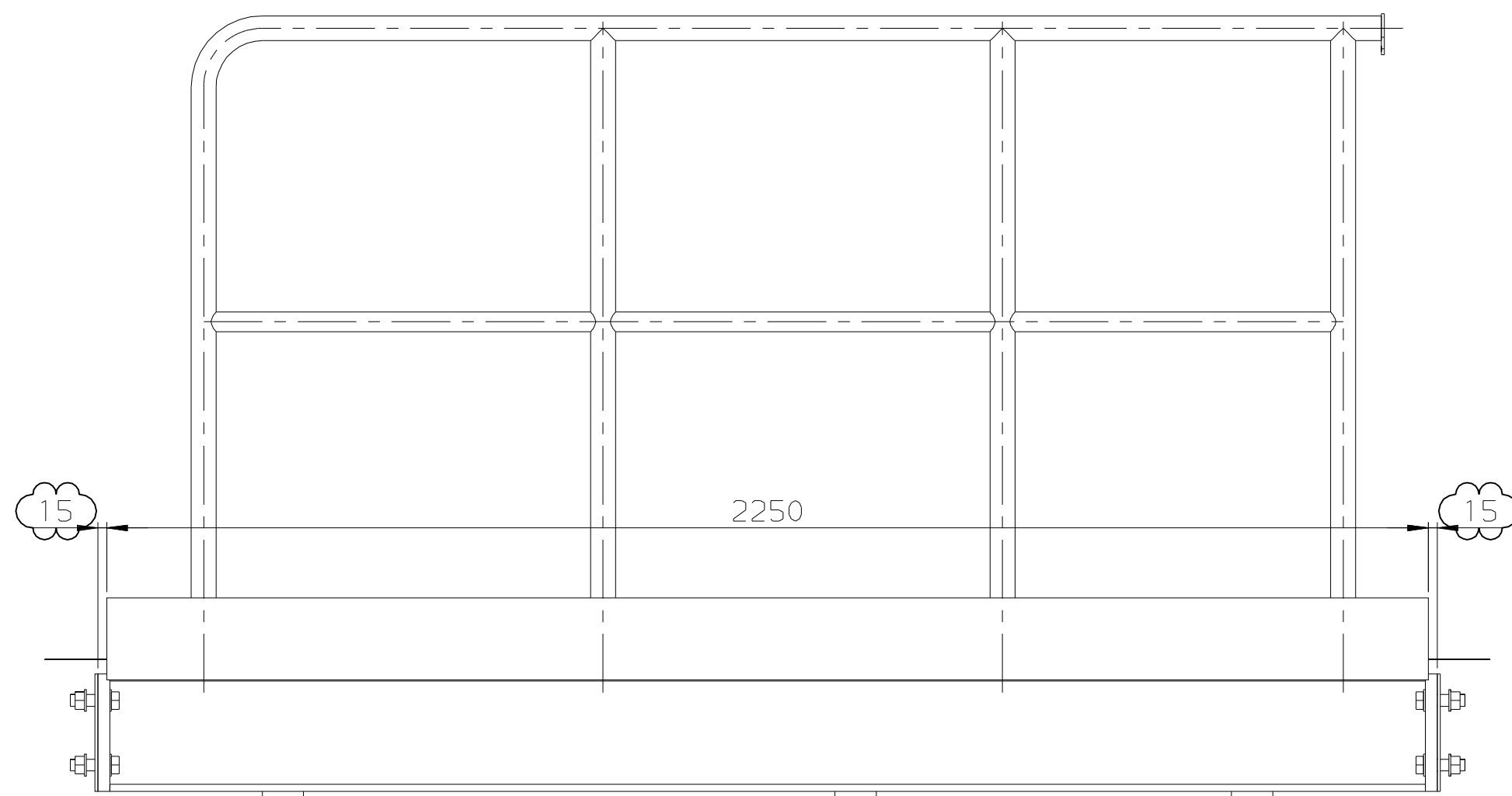
VIEW A
