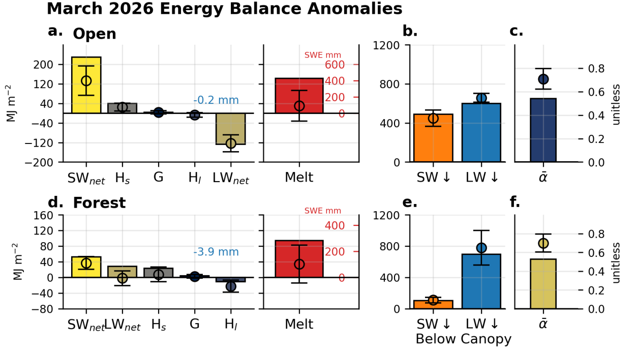
Figure 8. TODO: FIX SMALL BUG IN LW/SW and albedo averaging!! Accumulated snow energy fluxes ( SW_{net} , LW_{net} , H_s , H_l , G ), Melt, radiation forcings, ( SW \downarrow , LW \downarrow ), and weighted snow \bar{\alpha} for the open (a–c) and forest (d–f) sites for the duration of March 2026, restricted to times when SWE is present. Open circles and whiskers show the averages and one-standard deviation from the March SUMMA historical period (2000–2026). Equivalent units of mm of melt are displayed in red text on the right-hand side of the Melt panel. The under-canopy SW \downarrow and LW \downarrow are depicted in panel (e).
