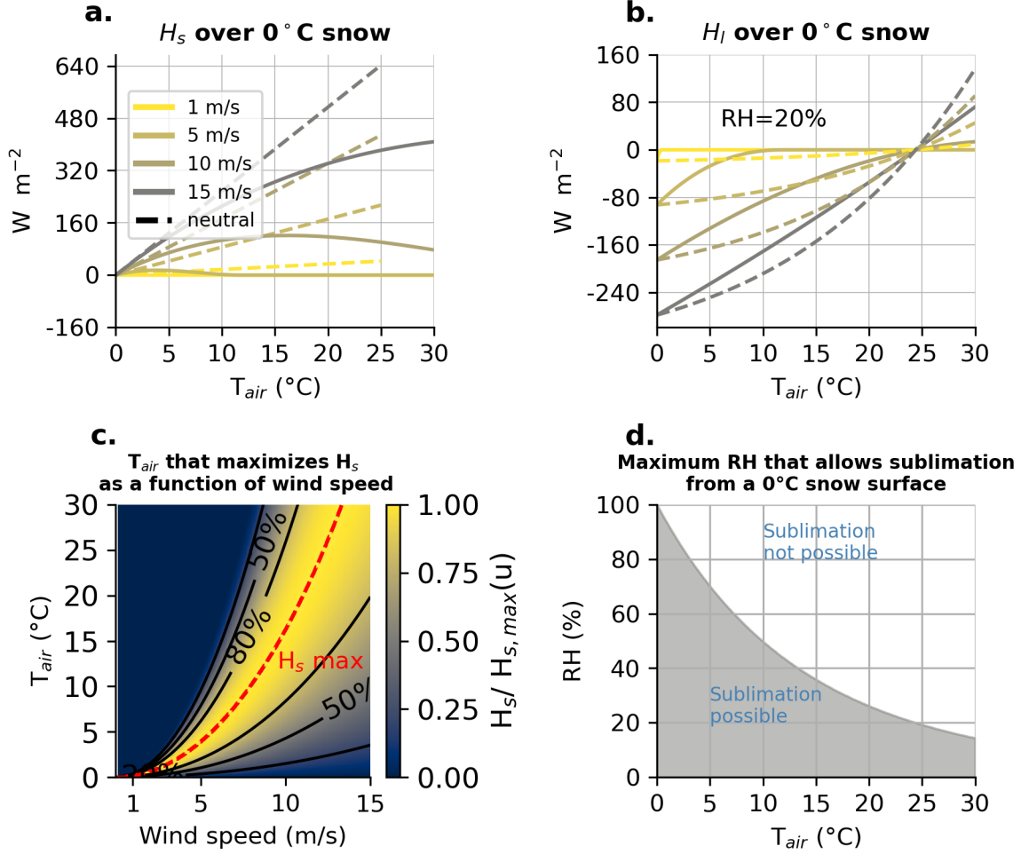
Figure 12. TODO: increase label size (a) Idealized sensible heat fluxes ( H_s ) into a melting snowpack as a function of T_{air} for four wind speeds (1, 5, 10, and 15 m\ s^{-1} ) at a 12 m height for open-conditions and a snow surface roughness of z_0=0.002 m. Dashed lines show flux assuming a neutral surface layer; solid lines show the same formulation with a stability correction applied as implemented in SUMMA. (b) the same as (a), but for H_l with a fixed RH of 20%. (c) The T_{air} that yields the maximum H_s into a 0°C snowpack after correcting for stability effects (dashed red line) for a given wind speed. Contours depict the fraction of the maximum H_s for that wind speed value. (d) The thermodynamic limitation of sublimation as a function of T_{air} , depicting the maximum RH that permits sublimation from a 0°C snowpack.
