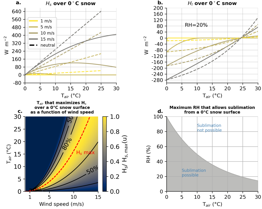
Figure 11. TODO: increase label size (a) Idealized sensible heat fluxes ( H_s ) into a melting snowpack as a function of T_{\text{air}} for four wind speeds (1, 5, 10, and 15 \text{m s}^{-1} ) at a 12 m height for open-conditions and a snow surface roughness of z_0=0.002 m. Dashed lines show flux assuming a neutral surface layer; solid lines show the same formulation with a stability correction applied as implemented in SUMMA. (b) the same as (a), but for H_l with a fixed RH of 20%. (c) The T_{\text{air}} that yields the maximum H_s into a 0 °C snowpack after correcting for stability effects (dashed red line) for a given wind speed. Contours depict the fraction of the maximum H_s for that wind speed value. (d) The thermodynamic limitation of sublimation as a function of T_{\text{air}} , depicting the maximum RH that permits sublimation from a 0 °C snowpack.
