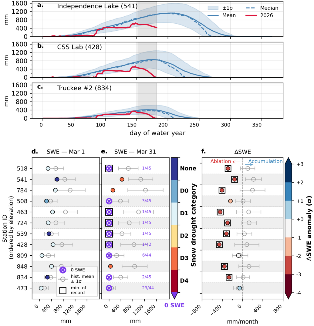
Figure 4. (a–c) Timeseries of SWE at three SNOTEL stations in the study region. The mean, median (dashed line), 1 standard-deviation (shaded region) and water year 2026 values are depicted. (d) SWE values on March 1st for the 12 SNOTEL sites in the study domain, labeled by their three-digit station code. (e) The same as (d), but for SWE on March 31. Color values depict the Hatchett et al. (2022) snow drought category. A 0 mm of SWE value is depicted by a purple circle marker. The purple text lists the number of 0 mm SWE occurrences observed on that date relative to the period of record for that site. (f) The SWE change between Mar 31 and Mar 1 ( \Delta SWE) compared with the historical record. Color values depict the deviation from the mean in units of standard deviation. Square markers bounding symbols indicate that the SWE or \Delta SWE is the record minimum for the period of record.
