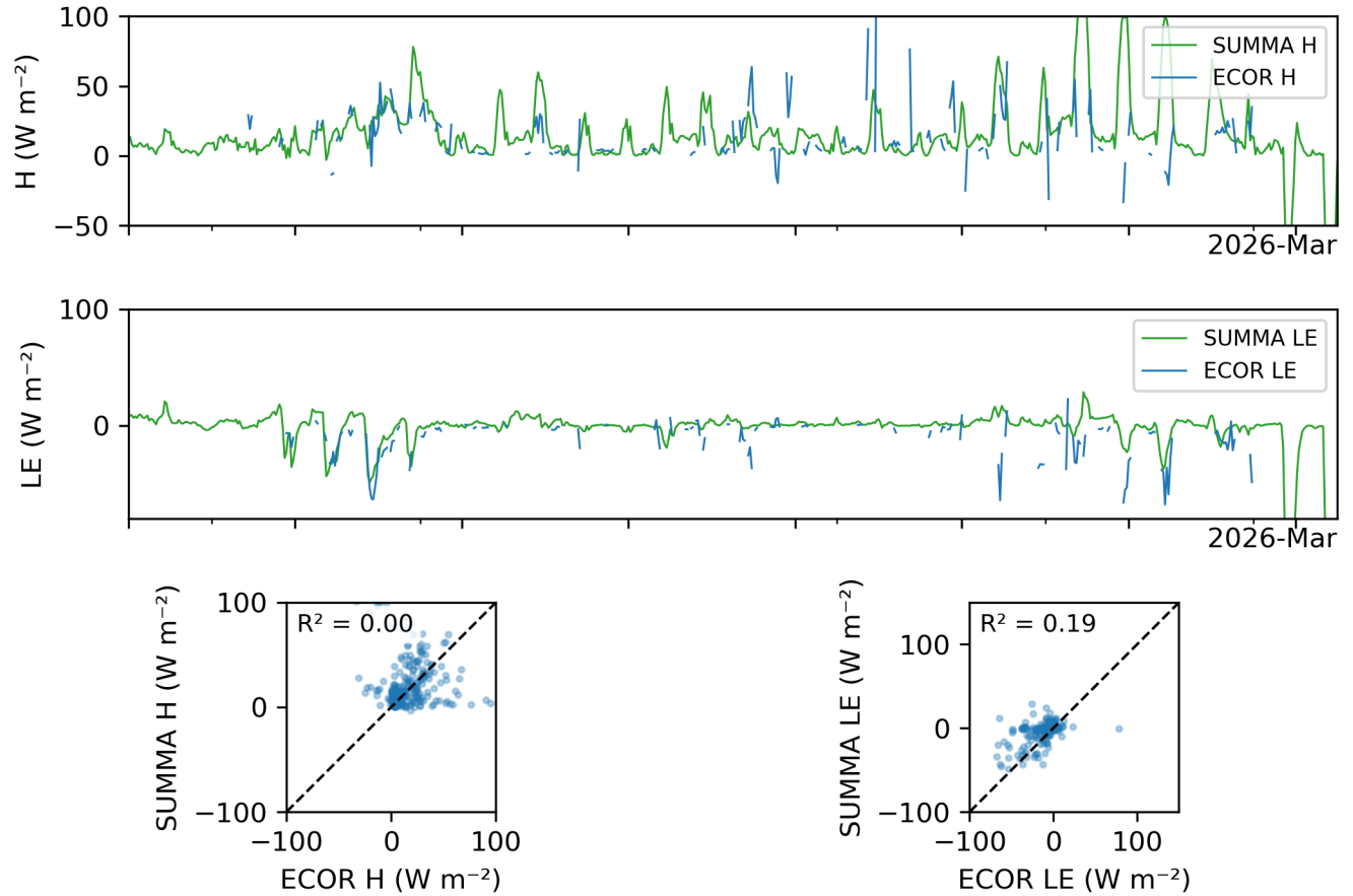
Figure S6: A comparison of SUMMA and eddy-covariance (ECOR) measured fluxes at CSSL for sensible heat ( H ) and latent heat ( LE ). The top shows a timeseries for the month of March 2026. The bottom two plots show 1:1 plots between the ECOR and SUMMA estimated fluxes.
