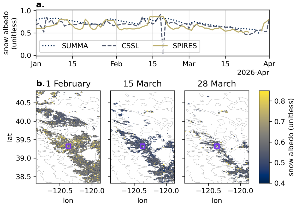
Figure S7: (a) SUMMA albedo evaluated against CSSL and SPIRES observations from 1 Jan 2026 to 1 April 2026. (b) Example maps of SPIReS snow albedo during water year 2026. CSSL is highlighted with the purple box. 500m elevation contours are depicted for reference.
