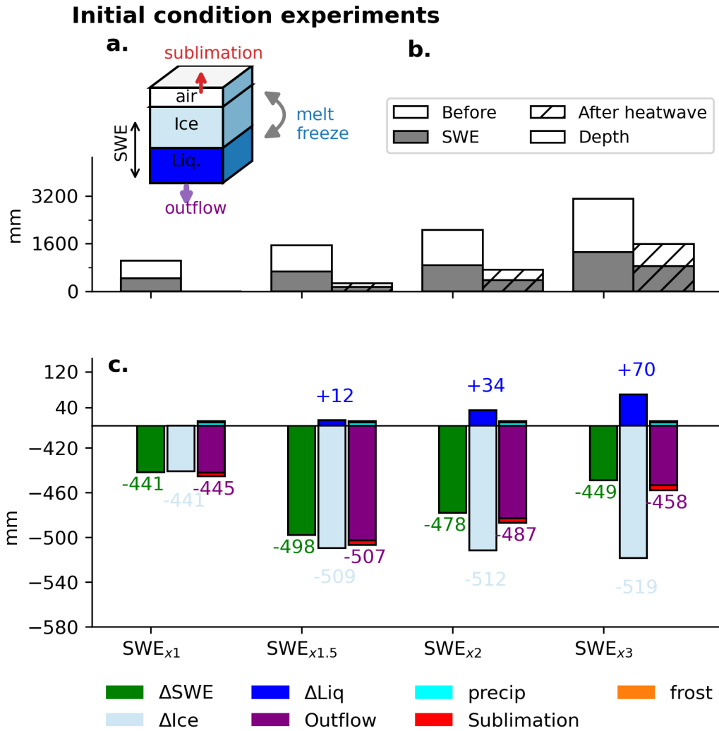
Figure S6: Initial condition tests. (a) a schematic of the snow mass balance composed of ice and liquid water, (b) the initial and final SWE and snow depth, and (c) mass components of the change in SWE for the different experiments.
