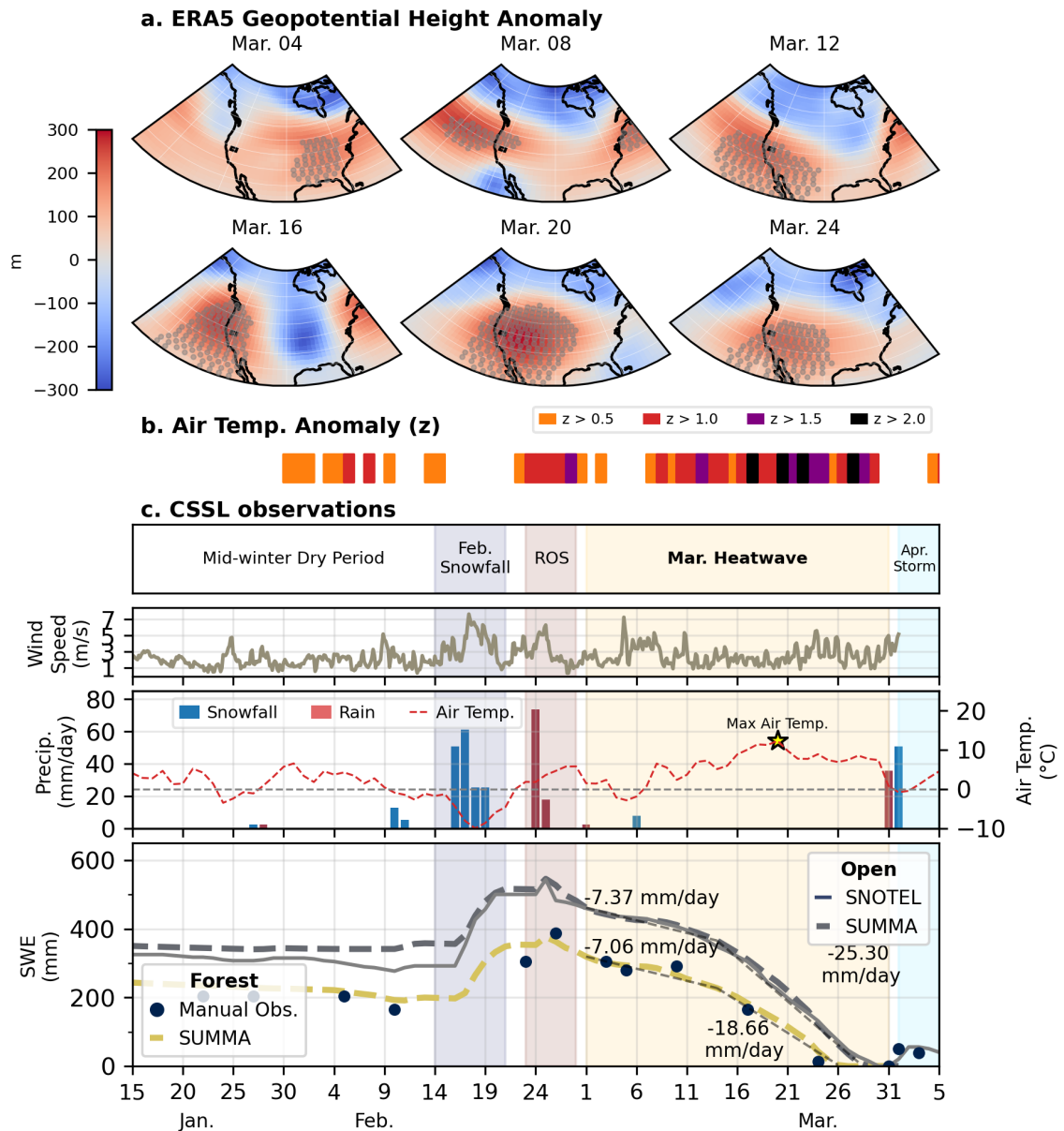
Figure 3. (a) The 500 mb geopotential height anomaly during the March 2026 heatwave from ERA5 for six days across the WUS. The study region is outlined using an overlain black rectangle. Gray stippling indicates regions with 500 mb geopotential height anomalies greater than 2- \sigma above the 1950-2022 mean for the month of March. (b-c) shows the time series of meteorological conditions at CSSL before and during the heatwave event. (b) depicts the daily average two-meter air temperature and daily precipitation rate. Days with a majority of rain (red) and a majority of snowfall (blue) are differentiated. (c) depicts the daily SWE and the one-day change in SWE (dSWE; right axis). Days with a positive dSWE (blue) are denoted by accumulation, and days with a negative dSWE (red) are termed melt days, acknowledging that some SWE may be lost by other processes.
