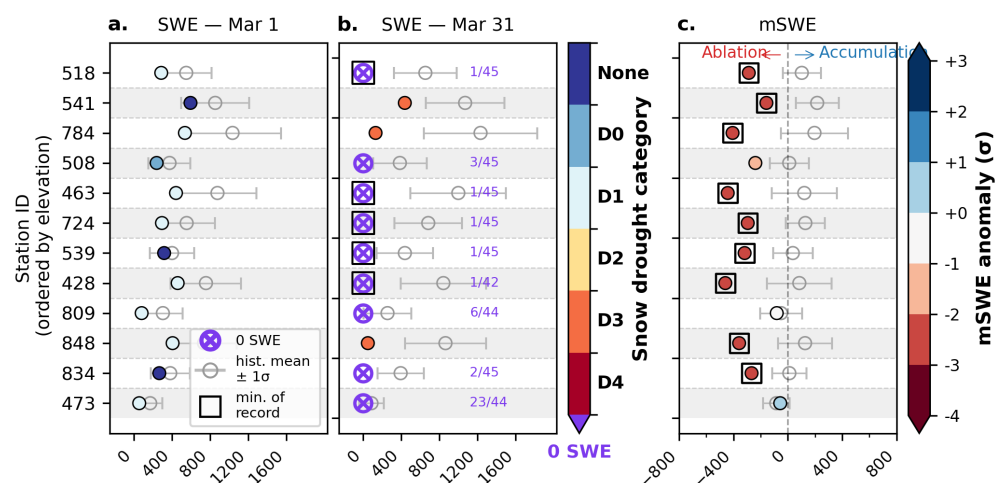
Figure 4. (a) SWE values on March 1st the 12 SNOTEL sites in the study domain, labeled by their three-digit station code. (b) The same as (a), but for SWE on March 31. Color values correspond with the snow drought D-scale. 0 SWE values are depicted by purple circle markers and the purple text lists how common 0 SWE was observed on that date for that site out of the period of record. (c) The SWE change between Mar 31 and Mar 1 (mSWE) compared with the historical record. Color values depict the deviation from the mean in units of standard deviation. Square markers bounding symbols indicates the SWE or mSWE is the record minimum for the period of record.
