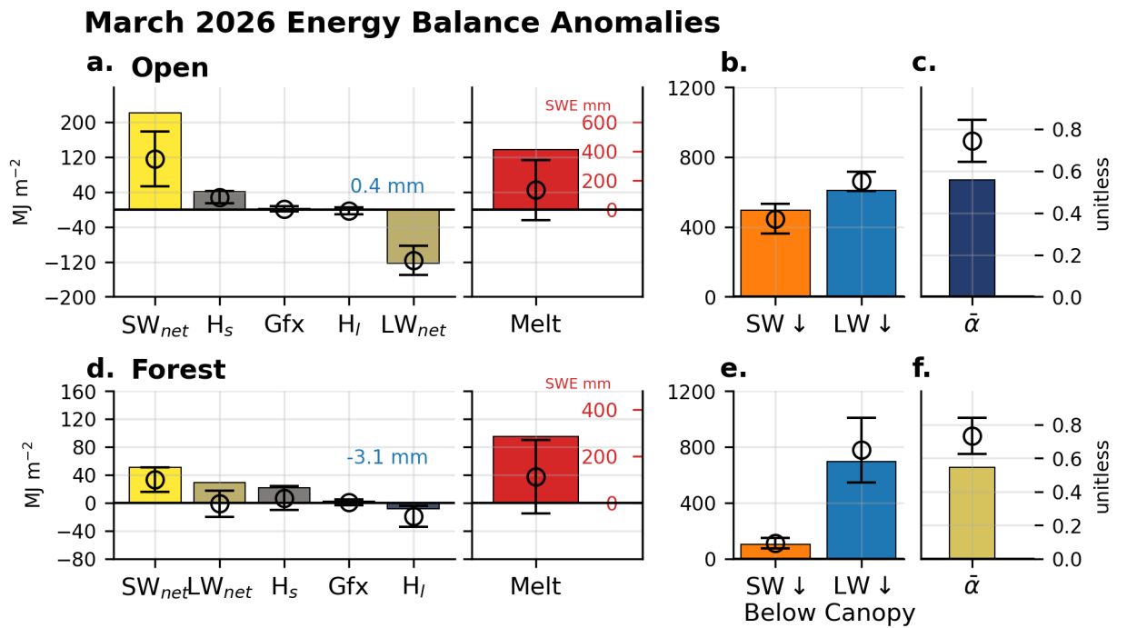
Figure 8. March-accumulated surface energy fluxes, snowmelt/cold-content responses, and snow albedo for the open (a–c) and forest (d–f) sites, restricted to hours with SWE > 4 mm. Solid bars gives the accumulated (or, for albedo, the incoming-shortwave-weighted mean) value for March 2026, and the adjacent boxplot (outliers omitted) shows the distribution of the same quantity across all March 1980–2025 water years. (a,d) Monthly-accumulated net shortwave ( SW_{net} ), net longwave ( LW_{net} ), sensible ( H_s ) and latent ( H_l ) heat, and ground heat flux ( G ) [ \text{MJ m}^{-2} ] for the open (a) and forest (d) sites; The inset in (a) shows the analogous accumulated SW \downarrow and LW \downarrow radiative forcing. (b,e) Accumulated total snowmelt energy (Melt) and change in snowpack cold content (dCC) for the open (b) and forest (e) sites. (c,f) Shortwave-weighted mean snow albedo ( \bar{\alpha} ) for the open (c) and forest (f) sites, computed by weighting each hour's albedo by its share of that month's total incoming shortwave radiation.
