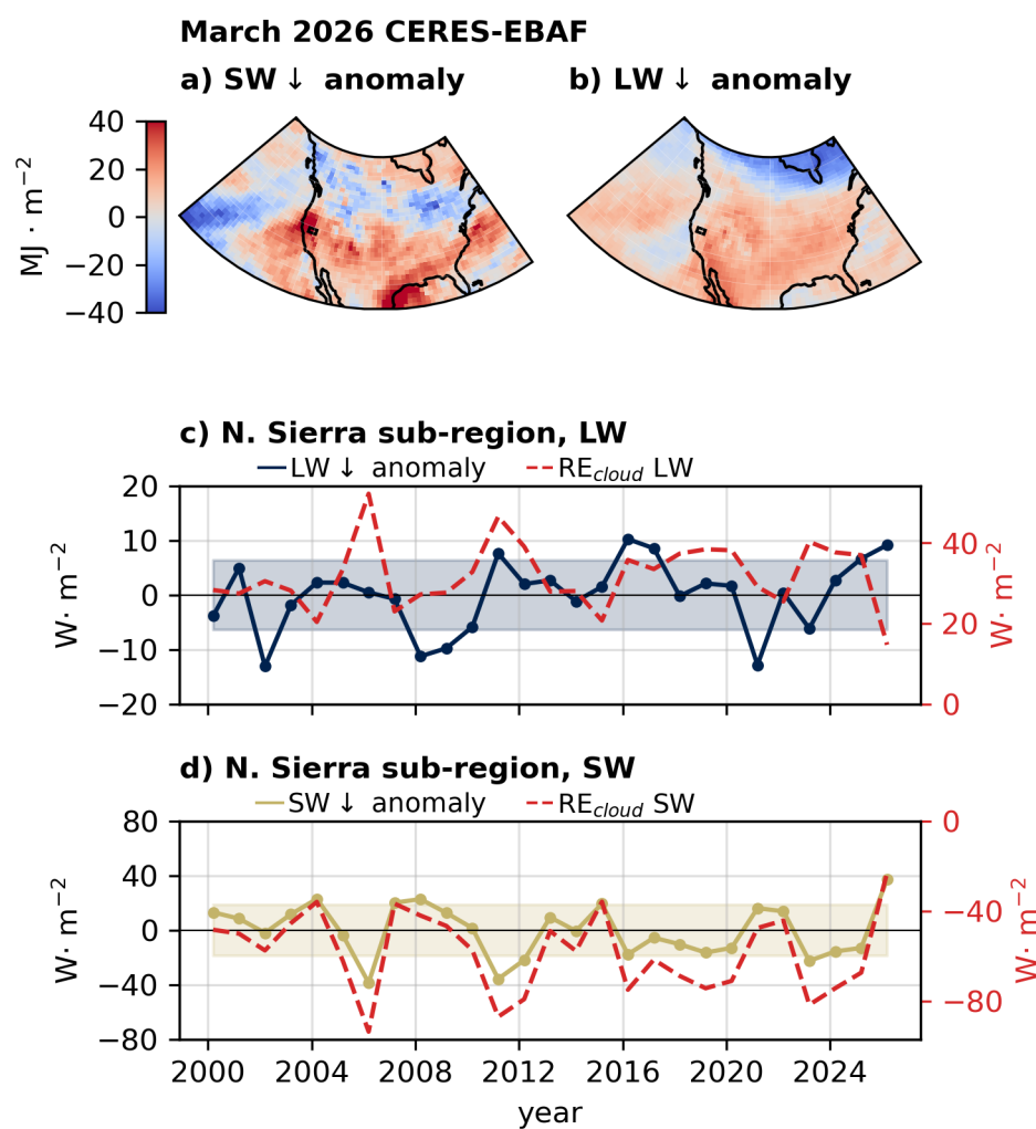
Figure 9. March SW \downarrow (a) and LW \downarrow (b) anomalies (relative to the March 2000 to present record) from the CERES EBAF 1x1 degree resolution product. (c) and (d) depicts the timeseries of anomalies averaged over the northern Sierra Nevada region in addition to cloud radiative effect amount (red), with units displayed on the right y-axis (in red-text). The shaded region in each plot depicts one standard deviation of the anomaly.
