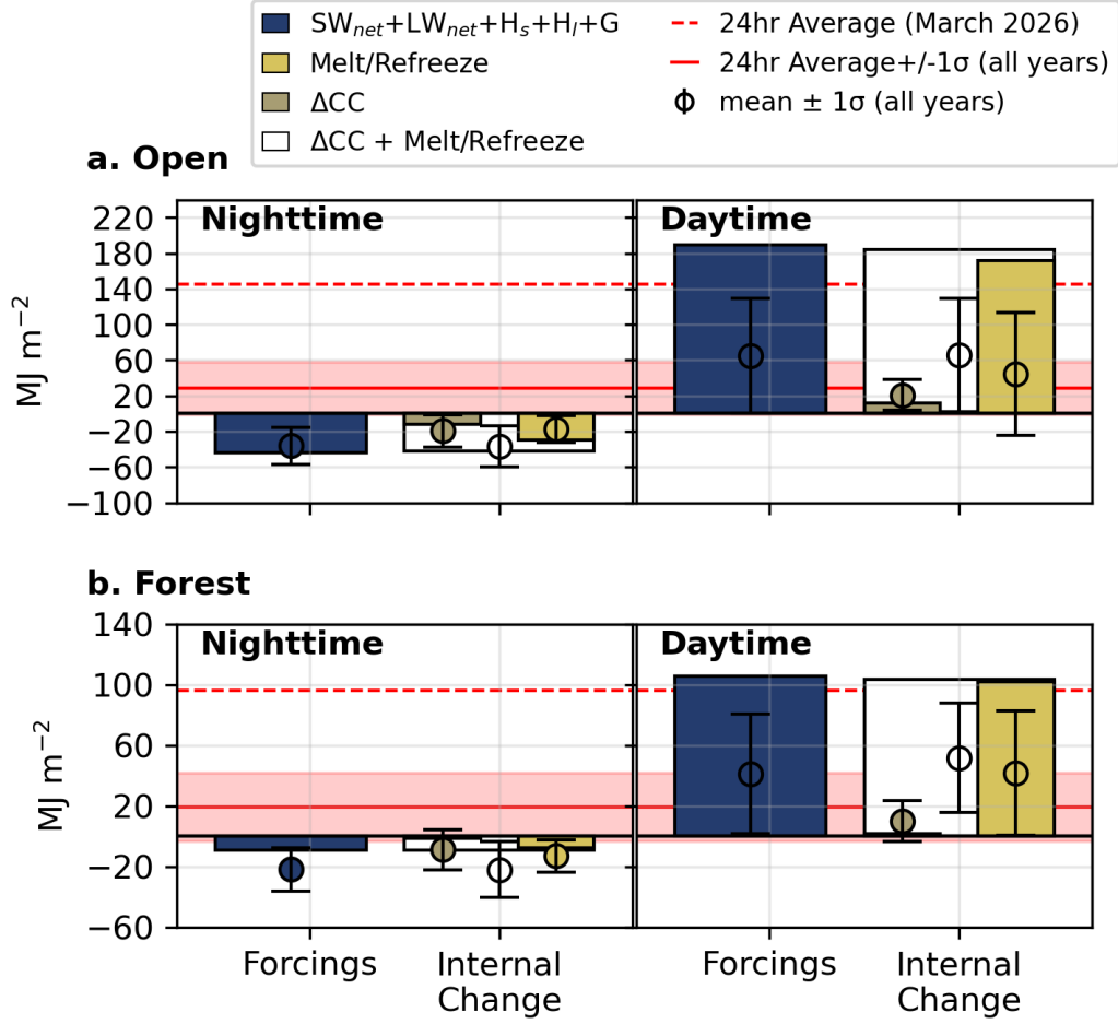
Figure 9. Similar to Fig. 8, but for daytime, nighttime, and 24hr 24-hour sums of accumulated energy balance components in the (a) open and (b) forest sites. Forcings include net-radiative and turbulent flux terms at top and bottom boundaries of the snowpack. Internal Change terms are the accumulated \Delta CC and Melt (positive) and Refreezing (negative) energy. \Delta CC and Melt/Refreeze are separated into individual terms for visualization purposes.
