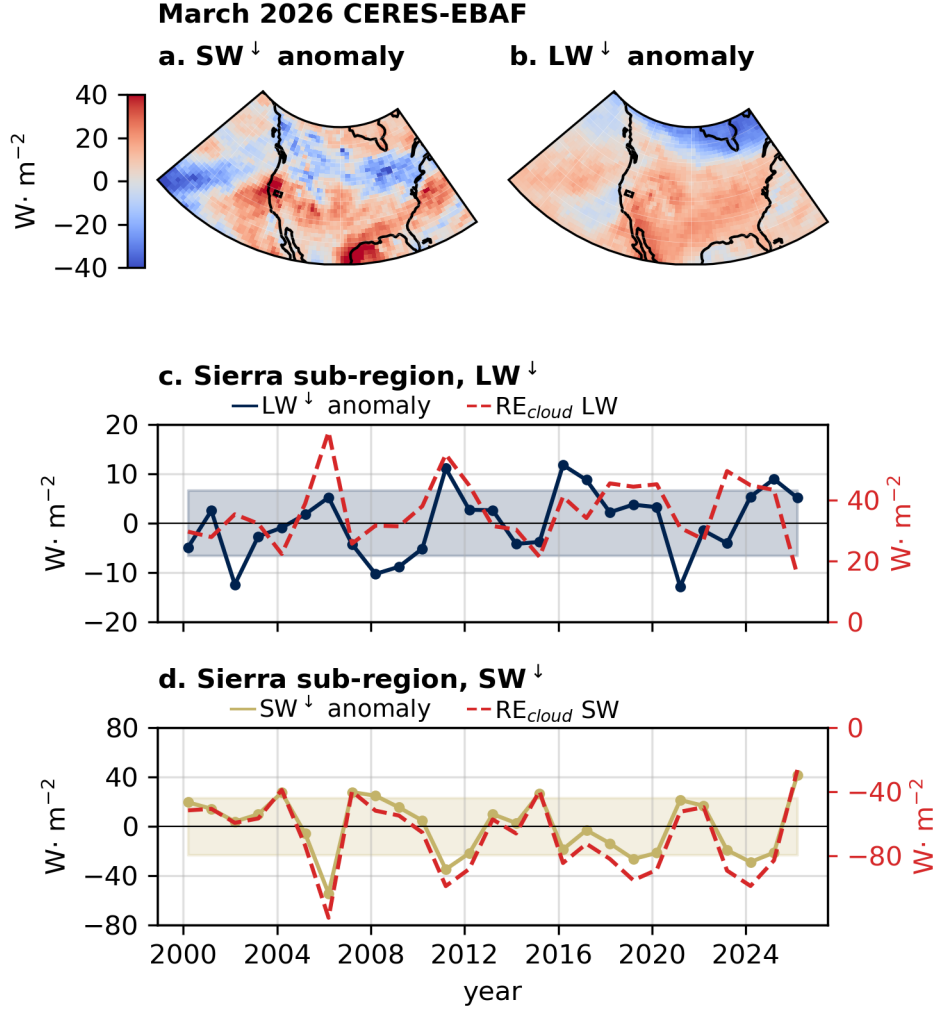
Figure 10. March SW^{\downarrow} (a) and LW^{\downarrow} (b) anomalies (relative to the March 2000 to present record) from the CERES-EBAF 1x1-degree 1^{\circ} \times 1^{\circ} resolution product. (c) and (d) depict the timeseries of anomalies averaged over the Sierra Nevada study region. RE_{cloud} amount is depicted with a twin y-axis, with units displayed on the right-hand side in red text. The shaded region in each plot depicts one standard deviation 1-\sigma of the anomaly.
