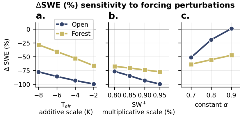
Figure 11. Sensitivity of \Delta SWE (%) from March 1 to March 31 to perturbations to (a) T_{air} and (b) SW^{\downarrow} forcings for open and forest sites. (c) shows the effect of proscribing prescribing a constant broadband snow \alpha .
