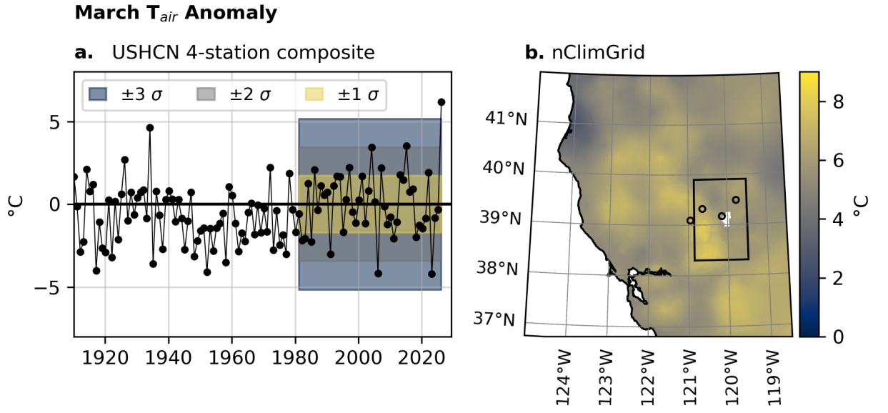
Figure 2. (a) Composite T_{\text{air}} anomalies from the four HCNv2 dataset stations in the greater Tahoe region study area for the month of March, from 1910 to 2026. Deviations and standard deviations with respect to the 1981–2010 mean T_{\text{air}} are depicted using shading. (b) The same, but for a map-view of the T_{\text{air}} anomaly of the gridded nClimGrid product. The box depicts the map boundary boundary from (Fig. 1b) and open circles depict USHCN station locations.
