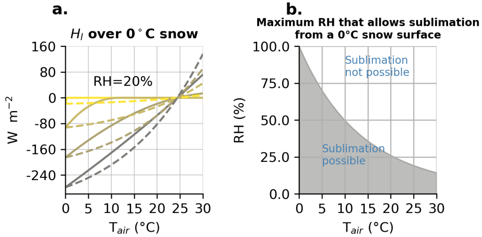
Figure 12. (a) Idealized latent heat fluxes ( H_l ) into a melting snowpack as a function of T_{air} for four wind speeds (1, 5, 10, and 15 m s^{-1} ) at a 12 m height for open-conditions and a snow surface roughness of z_0=0.002 m. Dashed lines show flux assuming a neutral surface layer; solid lines show the same formulation with a stability correction applied. Contours depict the fraction of the maximum H_s for that wind speed value. (b) The thermodynamic limitation of sublimation as a function of T_{air} , depicting the maximum RH that permits sublimation from a 0^{\circ}C snow-pack.
