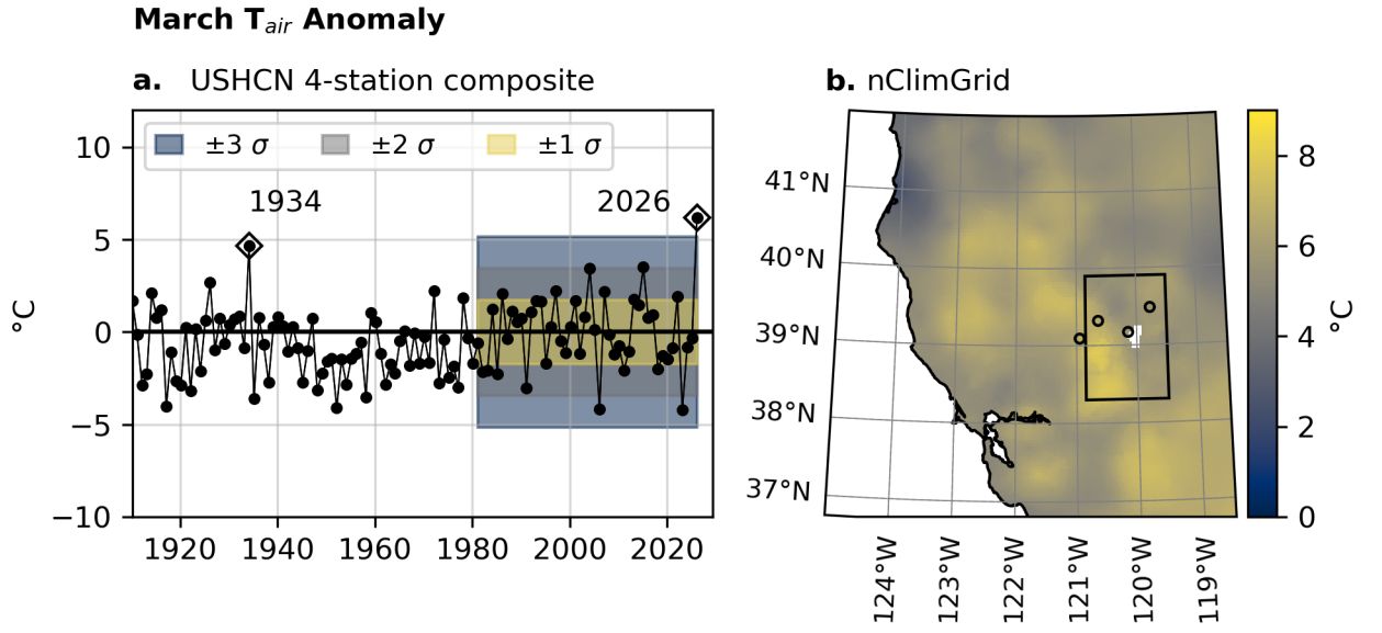
Figure 2. (a) Composite T_{air} anomalies from the four HCNv2 dataset stations in the greater central California Sierra Nevada region study area for the month of March, from 1910 to 2026. Deviations and standard deviations with respect to the 1981–2010 mean T_{air} are depicted using shading. (b) The same, but for a map-view of the T_{air} anomaly of the gridded nClimGrid product. The box depicts the map boundary from (Fig. 1b) and open circles depict USHCN station locations.
