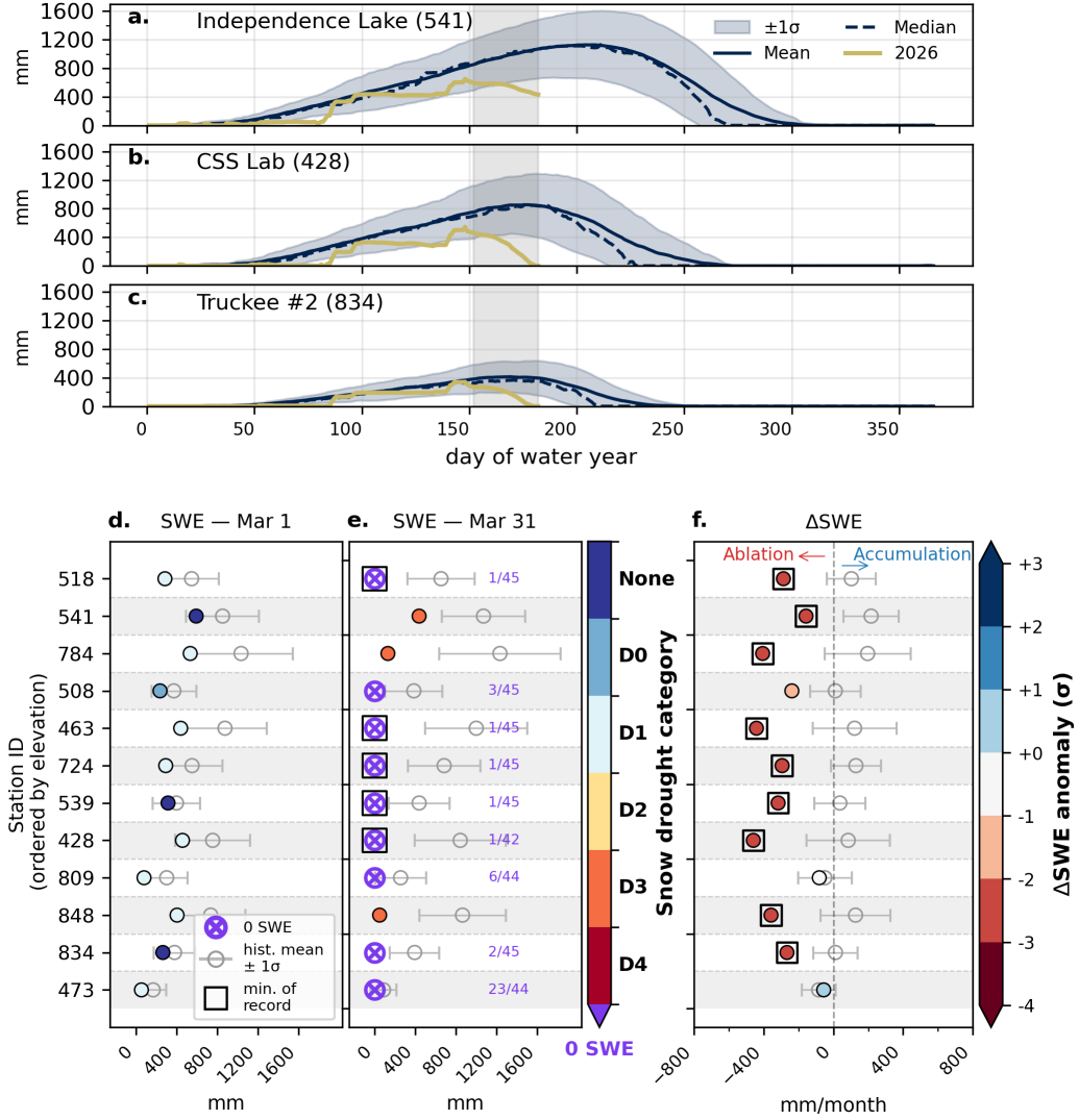
Figure 4. (a–c) Timeseries of SWE at three SNOTEL stations in the study region. The mean, median (dashed line), 1-\sigma (shaded region) and water year 2026 values are depicted. (d) SWE values on March 1st for the 12 SNOTEL sites in the study domain, labeled by their three-digit station code. (e) The same as (d), but for SWE on March 31. Color values depict the Hatchett et al. (2022) snow drought category. A 0 mm of SWE value is depicted by a purple circle marker. The purple text lists the number of 0 mm SWE occurrences observed on that date relative to the period of record for that site. (f) The SWE change between Mar 31 and Mar 1 ( \Delta SWE) compared with the historical record. Color values depict the deviation from the mean in units of \sigma . Square markers bounding symbols indicate that the SWE or \Delta SWE is the record minimum for the period of record.
