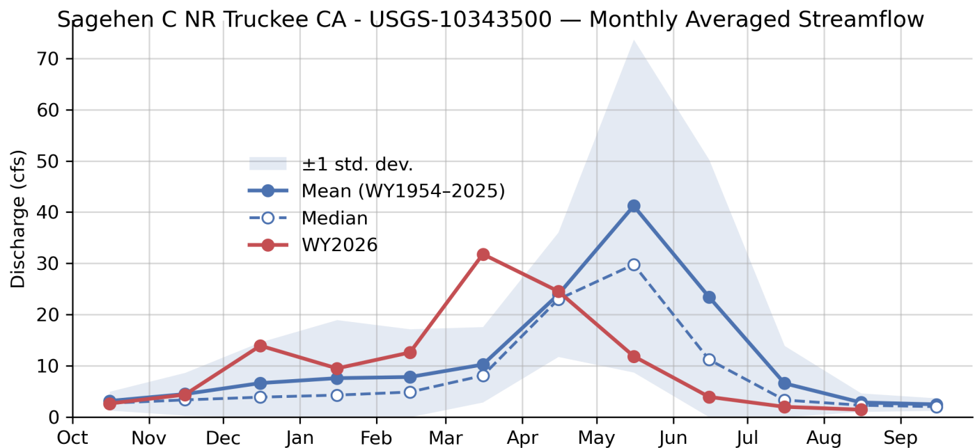
Figure S1: Monthly averaged streamflow in cubic feet per second (cfs) from 1954 to present for the USGS Sagehen Creek gage site. The historical mean, historical median, historical 1- \sigma range (shaded region), and WY2026 streamflow are depicted.
