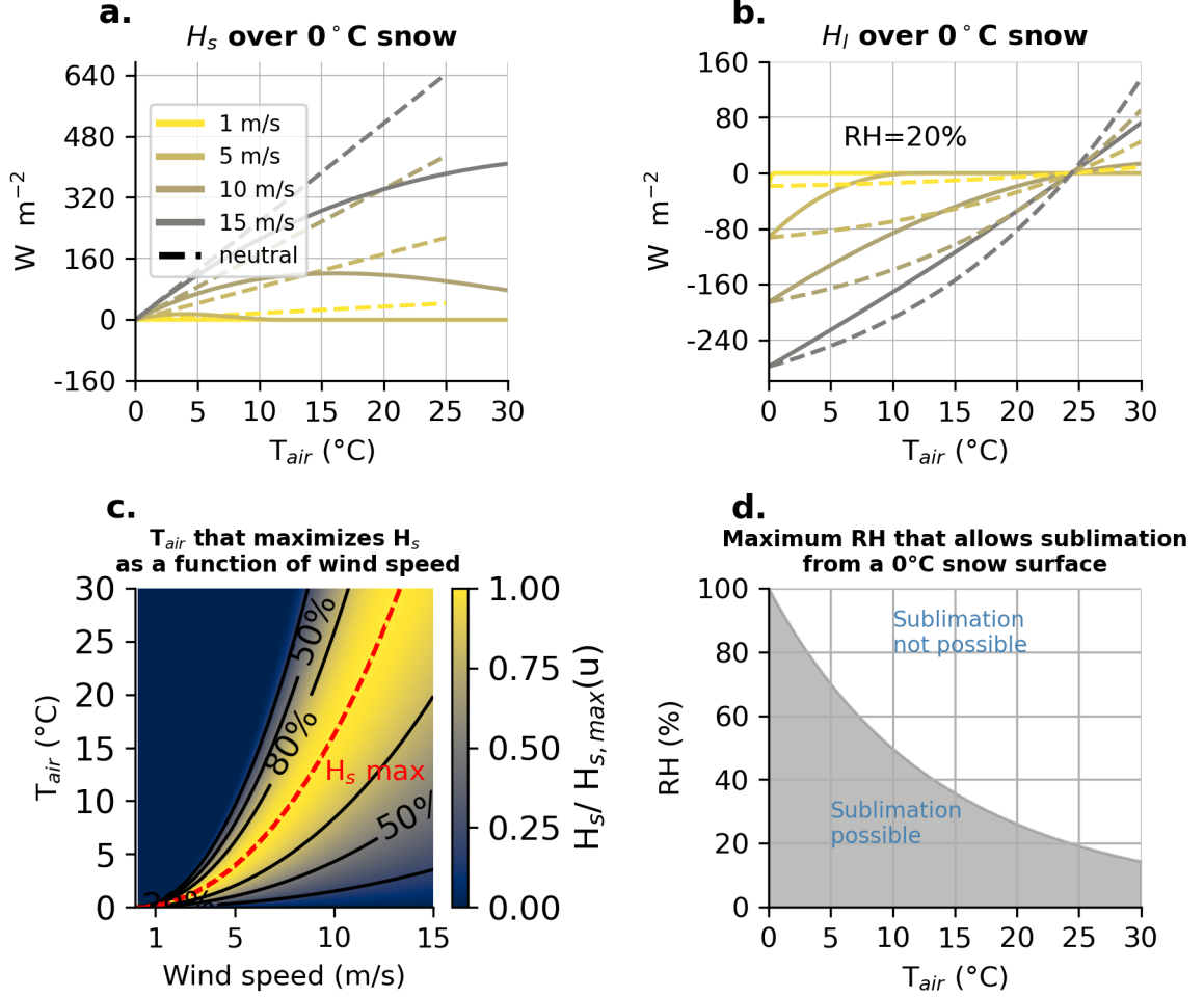
Figure 12. (a) Idealized sensible heat fluxes ( H_s ) into a melting snowpack as a function of T_{air} for four wind speeds (1, 5, 10, and 15 m\ s^{-1} ) at a 12 m height for open-conditions and a snow surface roughness of z_0=0.002\ m . Dashed lines show flux assuming a neutral surface layer; solid lines show the same formulation with a stability correction applied as implemented in SUMMA. (b) the same as (a), but for H_l with a fixed RH of 20%. (c) The T_{air} that yields the maximum H_s into a 0°C snowpack after correcting for stability effects (dashed red line) for a given wind speed. Contours depict the fraction of the maximum H_s for that wind speed value. (d) The thermodynamic limitation of sublimation as a function of T_{air} , depicting the maximum RH that permits sublimation from a 0°C snowpack.
