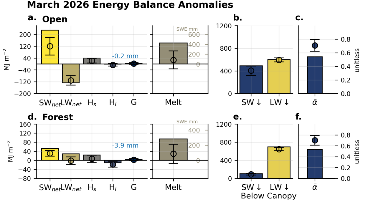
Figure 8. Accumulated snow energy fluxes ( SW_{net} , LW_{net} , H_s , H_l , G ), Melt, radiation forcings, ( SW^{\downarrow} , LW^{\downarrow} ), and weighted snow \bar{\alpha} for the open (a–c) and forest (d–f) sites for the duration of March 2026, restricted to times when SWE is present. Open circles and whiskers show the average and 1- \sigma from the March SUMMA historical period (2000–2026). Equivalent units of mm of melt are displayed in red text on the right-hand side of the Melt panels (a and d). The under-canopy SW^{\downarrow} and LW^{\downarrow} are depicted in panel (e).
