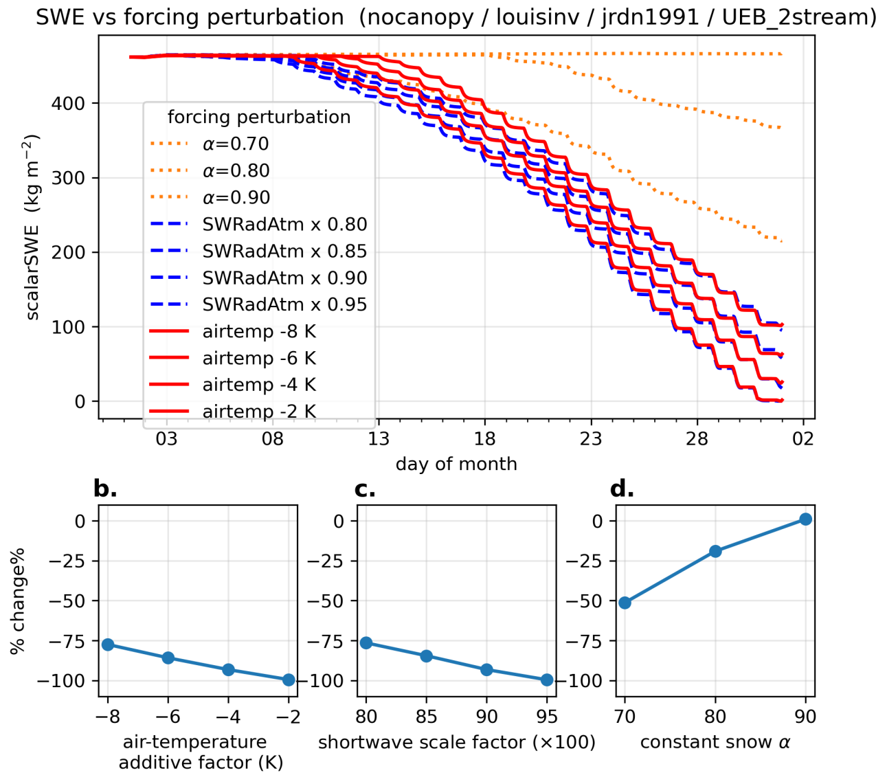
Figure S9: Sensitivity to perturbing model forcing variables.
