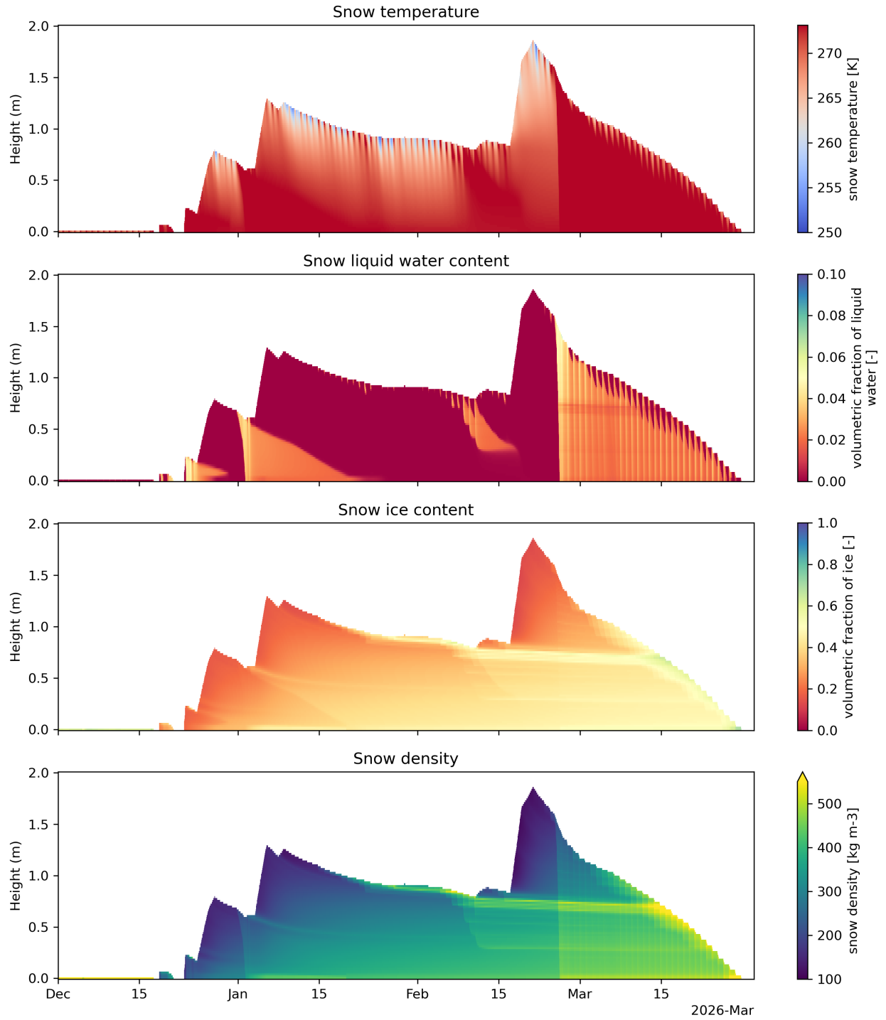
Figure S4: A timeseries of vertical cross-sections of snow temperature, snow liquid water content volumetric fraction, snow ice content volumetric fraction, and snow density (bottom) during the accumulation season
