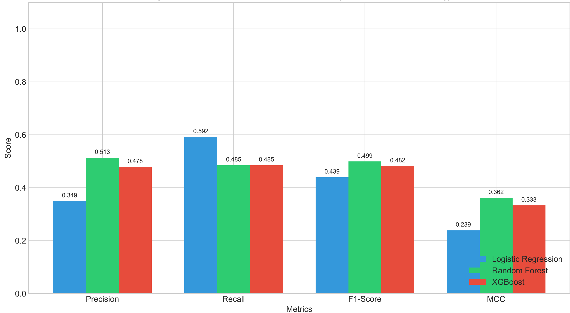
Figure 5: Model Performance Comparison (After SMOTE Balancing)
