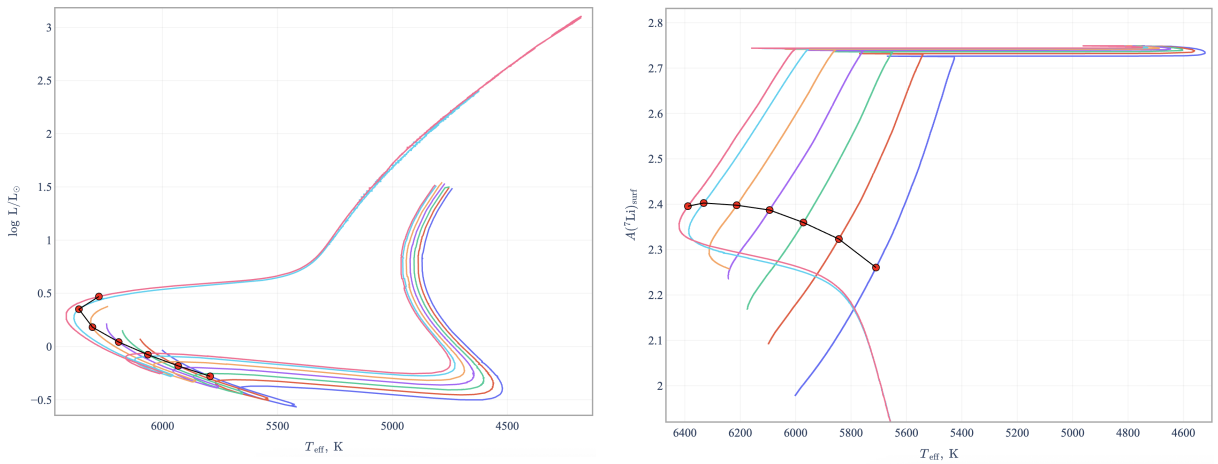
Figure 8: Left: HRDs for 7 models with the same chemical composition and physics (colored lines) and an isochrone at the age of 12.5 Gyr (black line connecting red circles). Right: Isochrone at the age of 10 Gyr for the same models in the A(\text{Li}) - T_{\text{eff}} diagram.
