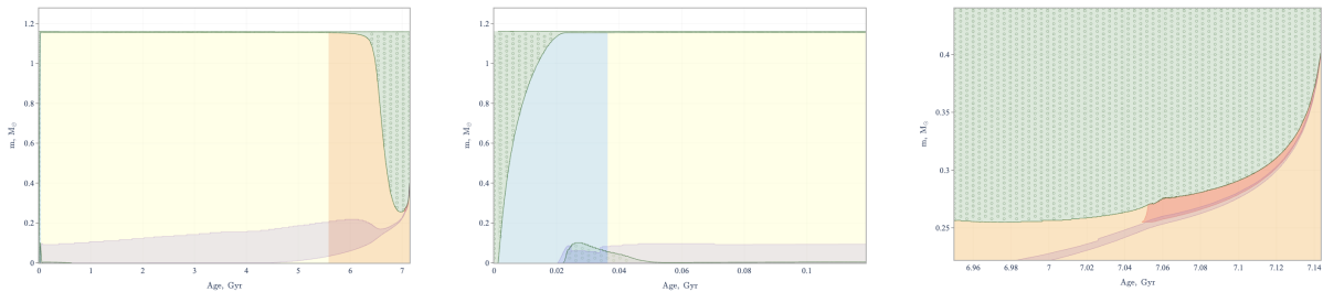
Figure 11: Left : Kippenhahn diagram for a star with mass of 1.16M_{\odot} (general view). Middle : zoom onto the Pre-main Sequence and early Main Sequence region. Right : zoom onto the bottom of the convective envelope (green area with rings) and thermohaline mixing zone (reddish area).
