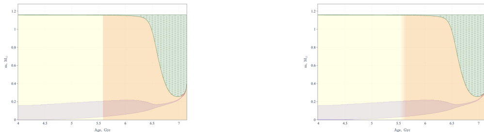
Figure 12: Kippenhahn diagram with sharp ( left ) and smooth transition ( right ) between phases.
