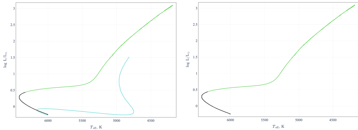
Figure 9: Left : HR diagram with Show phase enabled. Right : The same as in the left panel, but with min phase set to 2 (Main Sequence), thus not showing the Phase 1 (Pre-Main Sequence).
