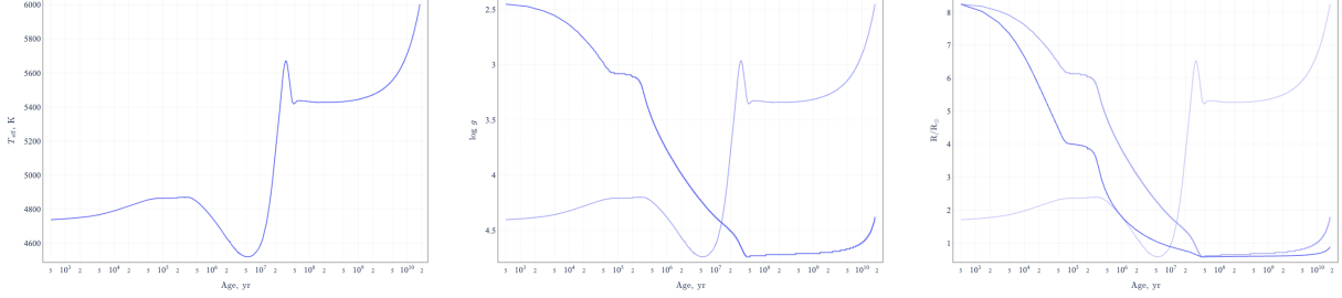
Figure 10: Left: T_{\text{eff}} -Age plot before the freeze. Middle: The same as in the left panel, but with \log g -Age overplotted. Right: The same as in the middle panel, but with R/R_{\odot} overplotted.
