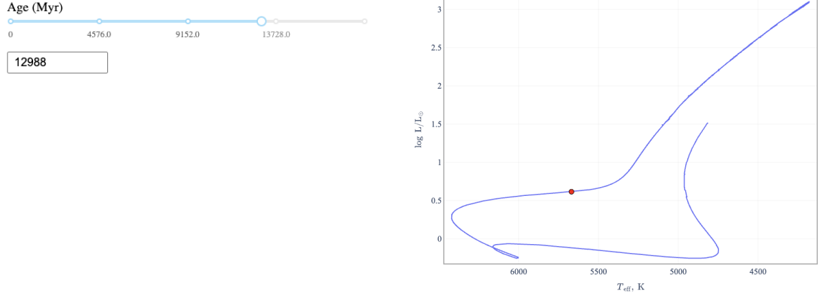
Figure 7: Left: Age slider. Right: HR diagram with a red circle point at the selected age.
