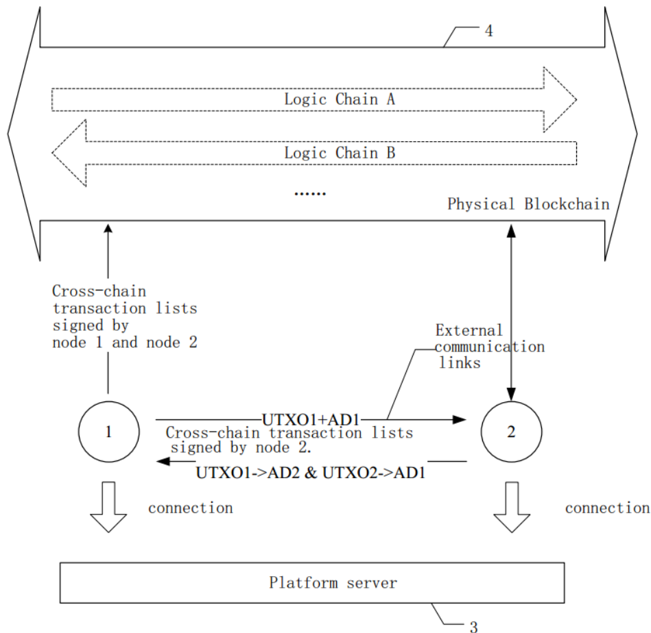
The diagram of patent method for Cross-chain Trading.
