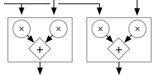
Parallel vector engines (NVDLA-like)
