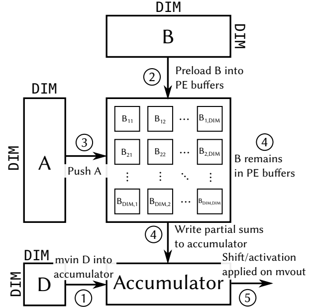
(b) In the Weight Stationary dataflow, the weight matrix B is preloaded and remains stationary in the PEs to maximize weight reuse.
