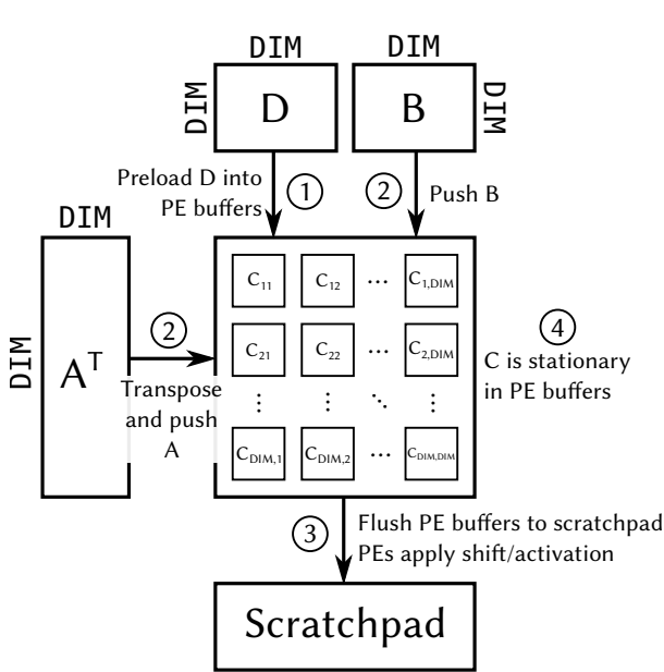
(a) In the Output Stationary dataflow, the result matrix C remains stationary in the PEs to accumulate partial sums.
