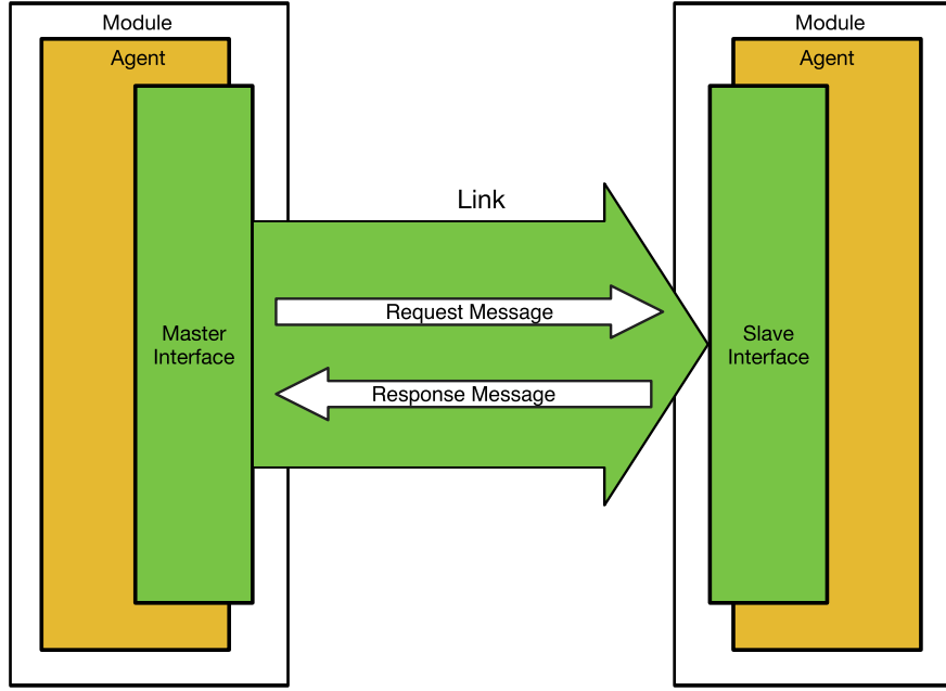
Figure 3.8: TileLink TL-UL connection structure. [24]
