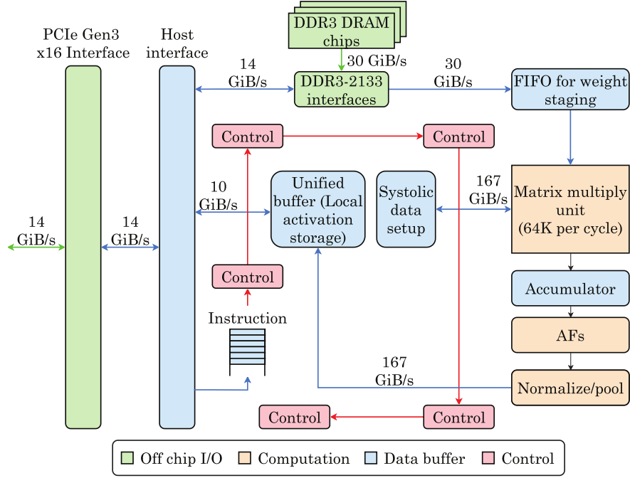
Figure 4.4: A high-level block diagram of the Google TPUv1. The design is dominated by the systolic Matrix Multiply Unit and its large on-chip Unified Buffer. [14, 20].
