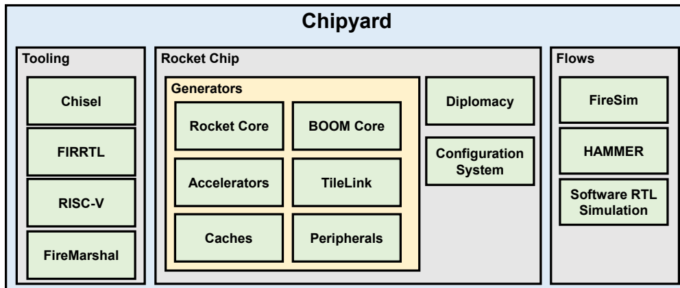
Figure 2.13: Component structure of Chipyard. [32]
