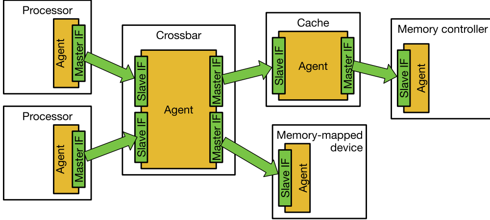
Figure 3.6: Connection model in TileLink and its interfaces. [24]
