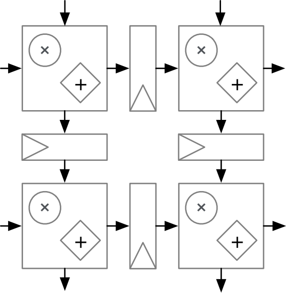
Systolic spatial array (TPU-like)
