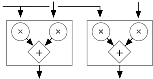
Parallel vector engines (NVDLA-like)
