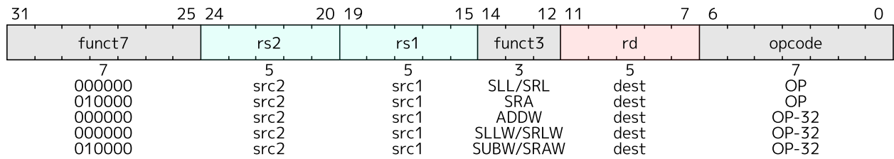
Figure 2.7: Encoding format for 64-bit R-type shift instructions for word operations. [30]
