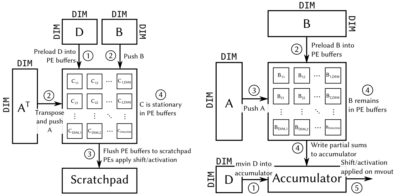
(a) In the Output Stationary dataflow, the result matrix C remains stationary in the PEs to accumulate partial sums.
