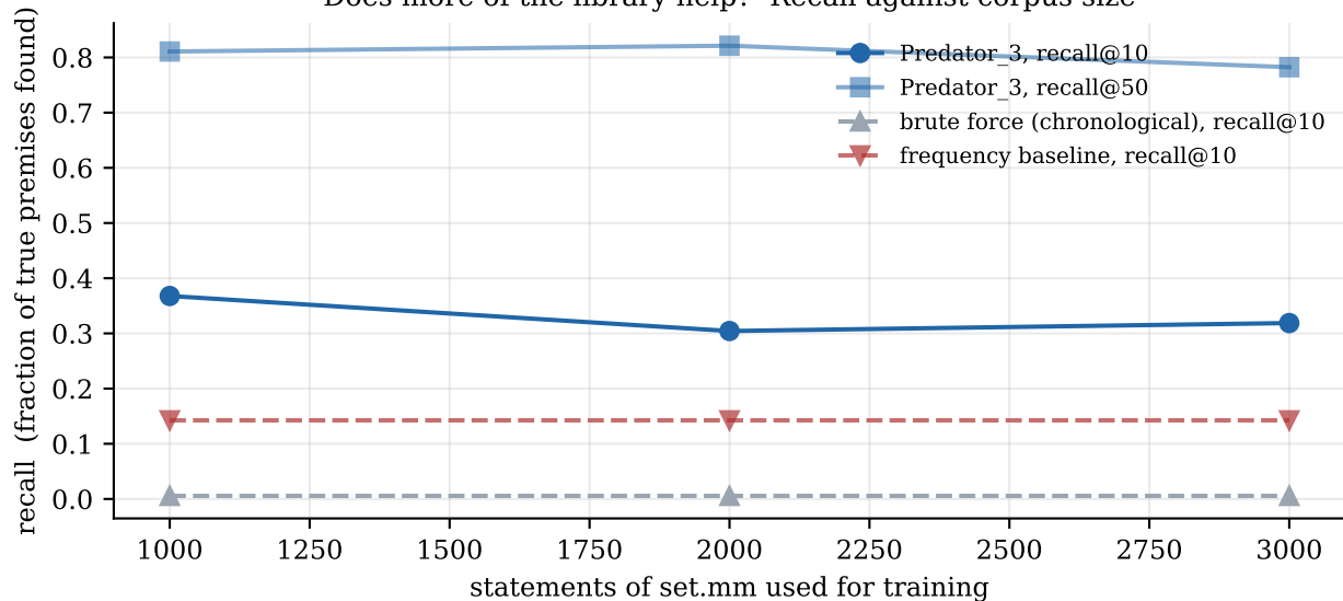
Does more of the library help? Recall against corpus size
