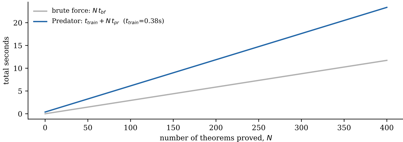
Training never amortises at this scale: the lines diverge
