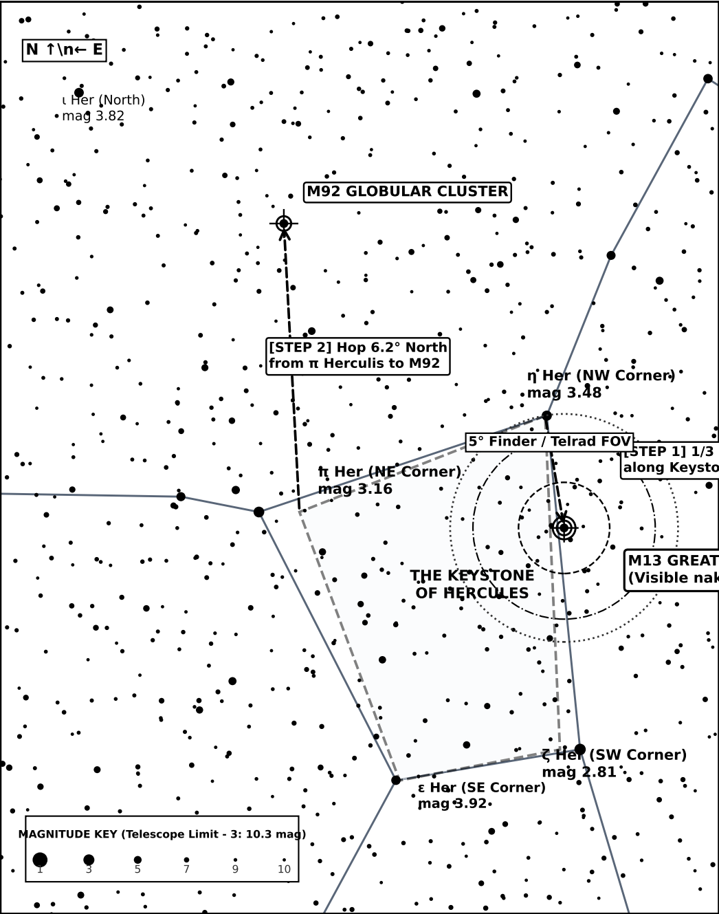
VIEWPORT A: WIDE-FIELD STAR-HOPPING CHART (Upright Naked-Eye / Finder: N ↑, E ←)
