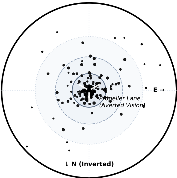
VIEWPORT B: EYEPIECE SIMULATION (Negative Inverted 180°: N ↓, E →)
