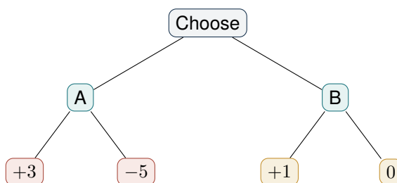
Figure 8.1: Minimax compares A's worst leaf -5 with B's worst leaf 0 , so it chooses B.
