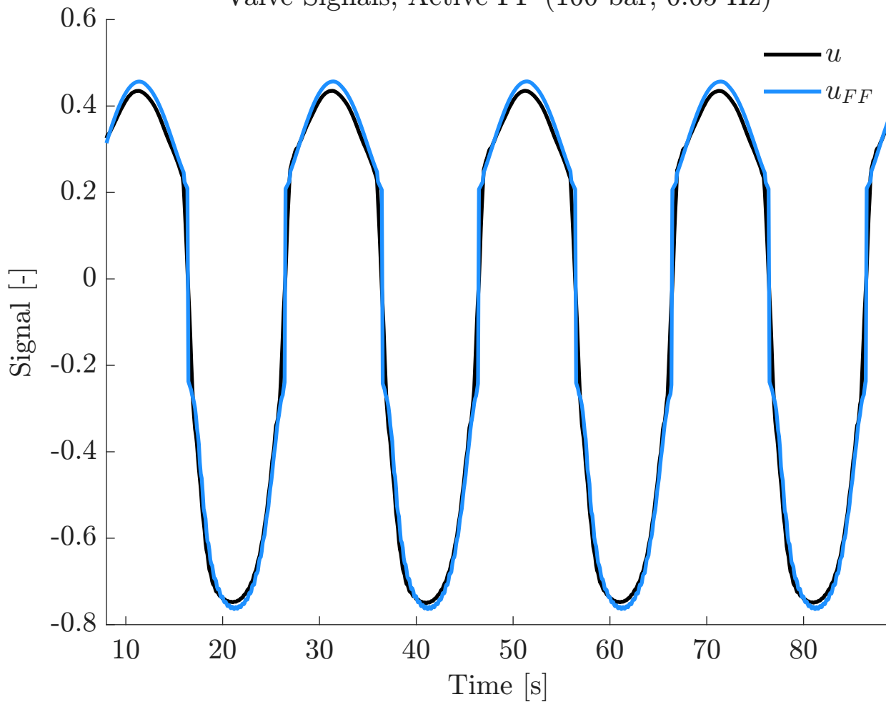
Valve Signals, Active FF (100 bar, 0.05 Hz)
