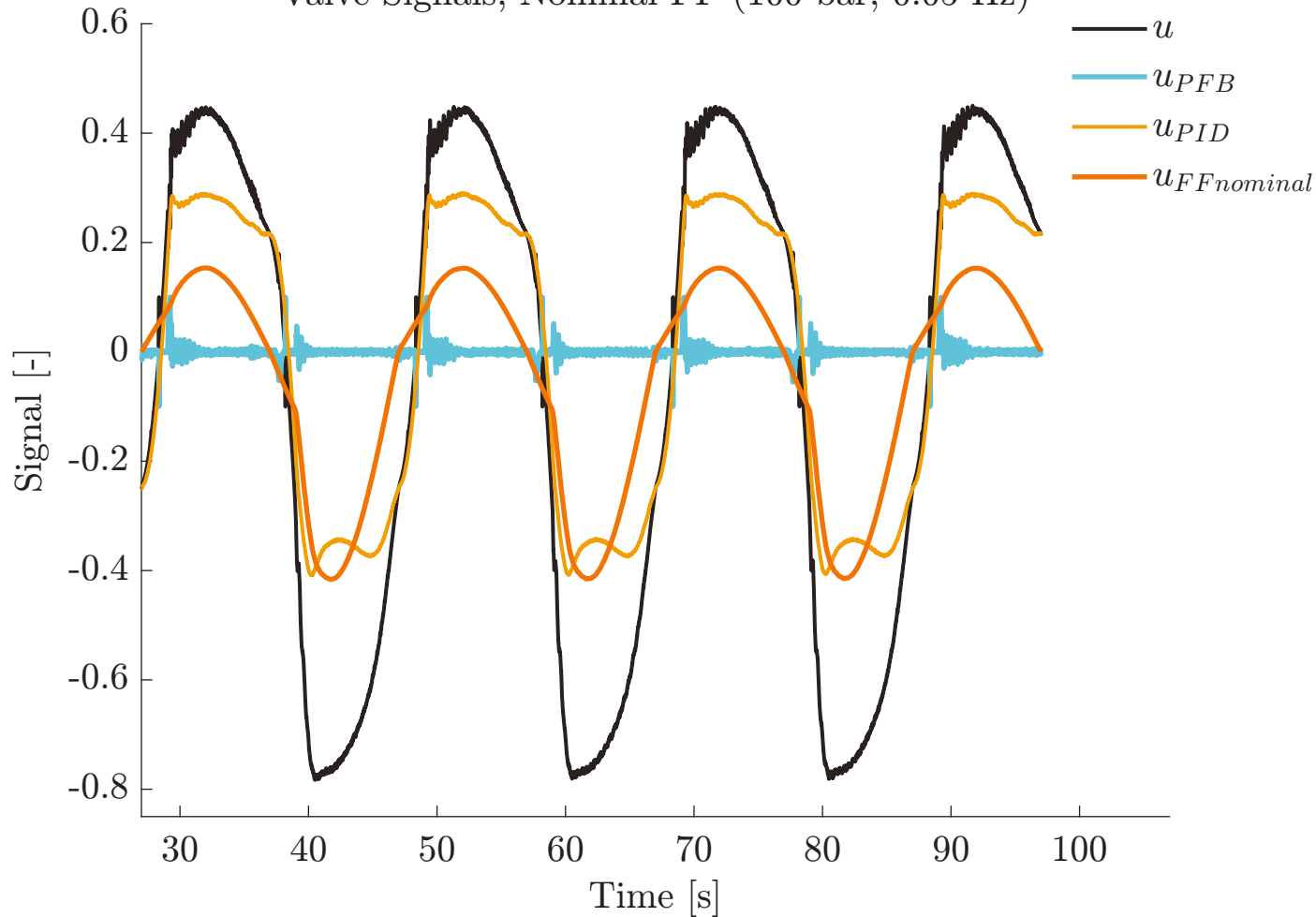
Valve Signals, Nominal FF (100 bar, 0.05 Hz)
