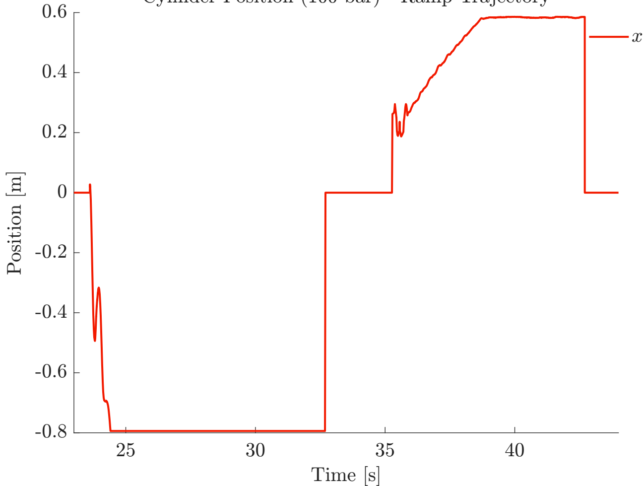
Cylinder Position (100 bar) - Ramp Trajectory
