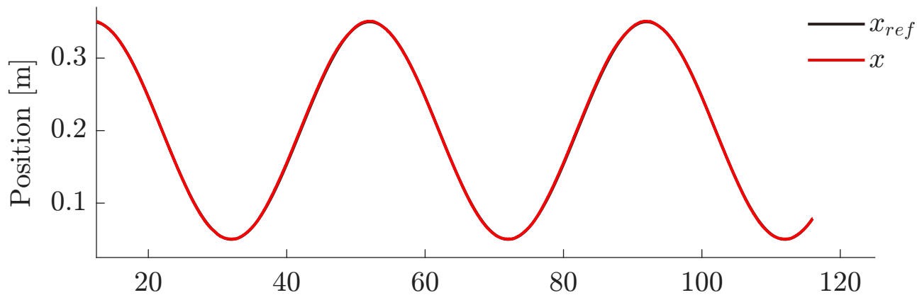
Active Kv FF (120 bar, 0.025 Hz)
