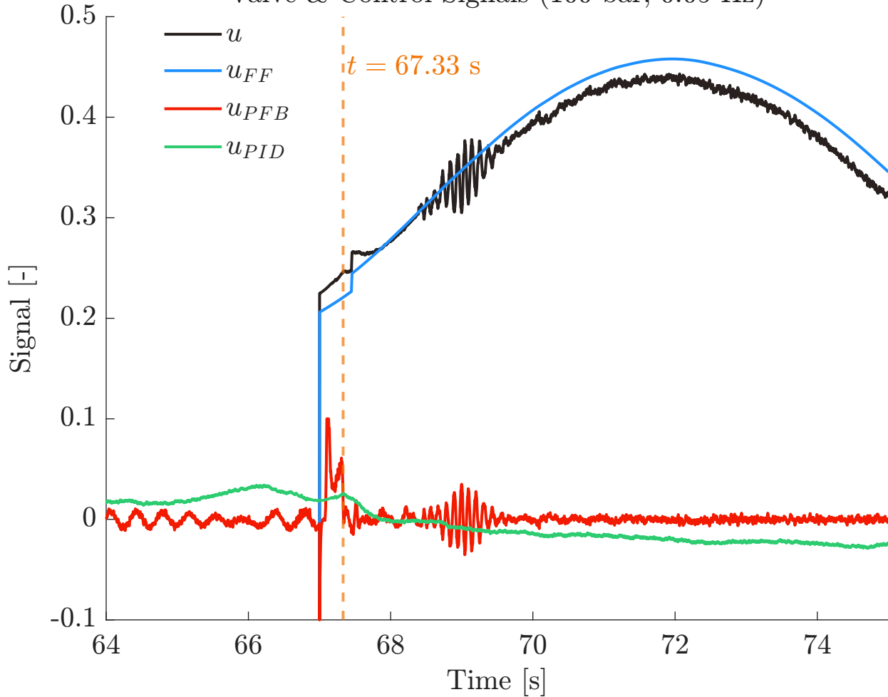
Valve & Control Signals (100 bar, 0.05 Hz)
