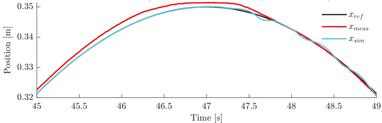
Position Tracking - Measured vs. Simulated (100 bar, 0.05 Hz)
