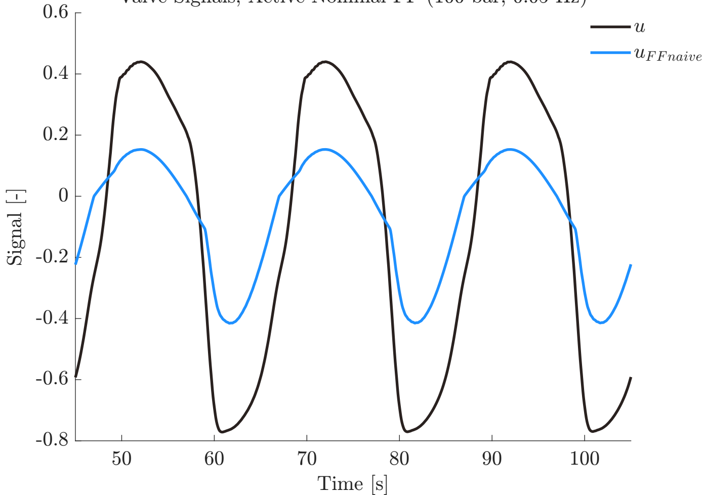
Valve Signals, Active Nominal FF (100 bar, 0.05 Hz)
