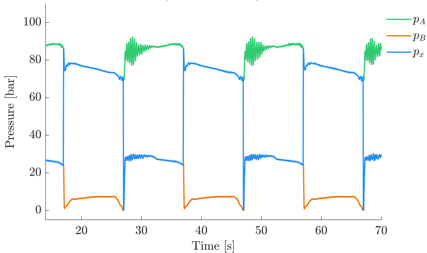
Pressure Feedback (120 bar, 0.05 Hz) - Selected Pressure
