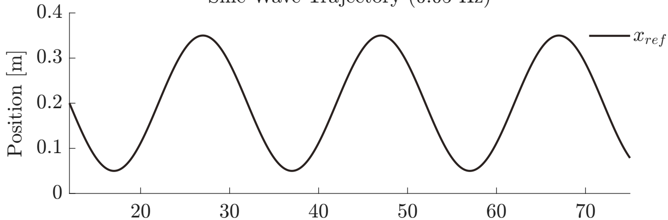
Sine Wave Trajectory (0.05 Hz)
