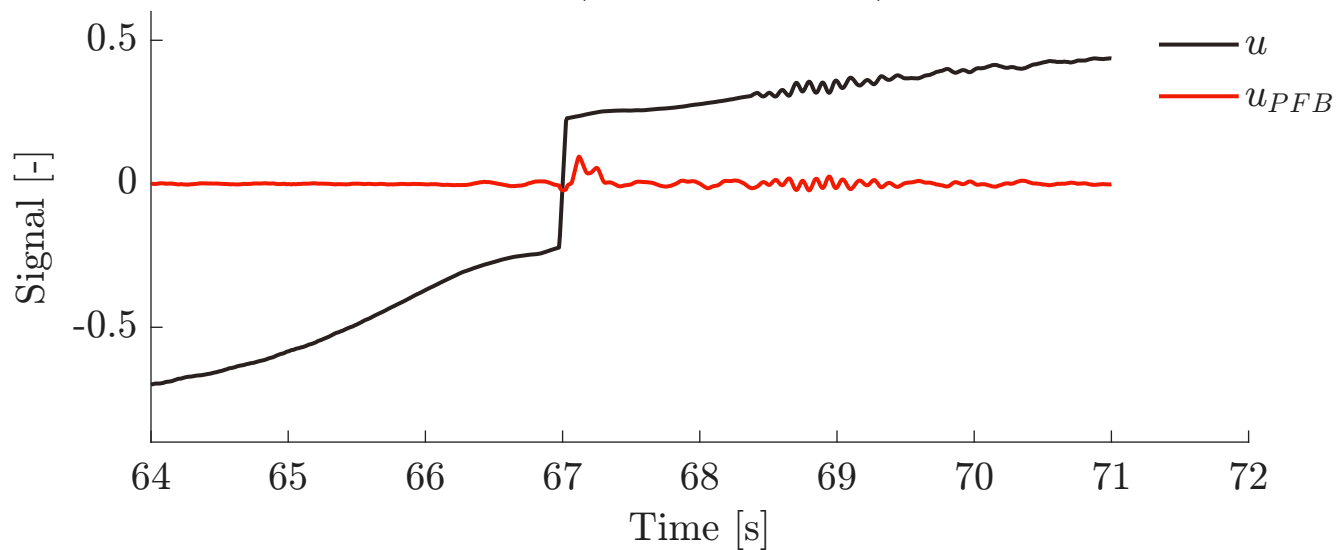
Pressure Feedback (100 bar, 0.05 Hz) - Valve Signals
