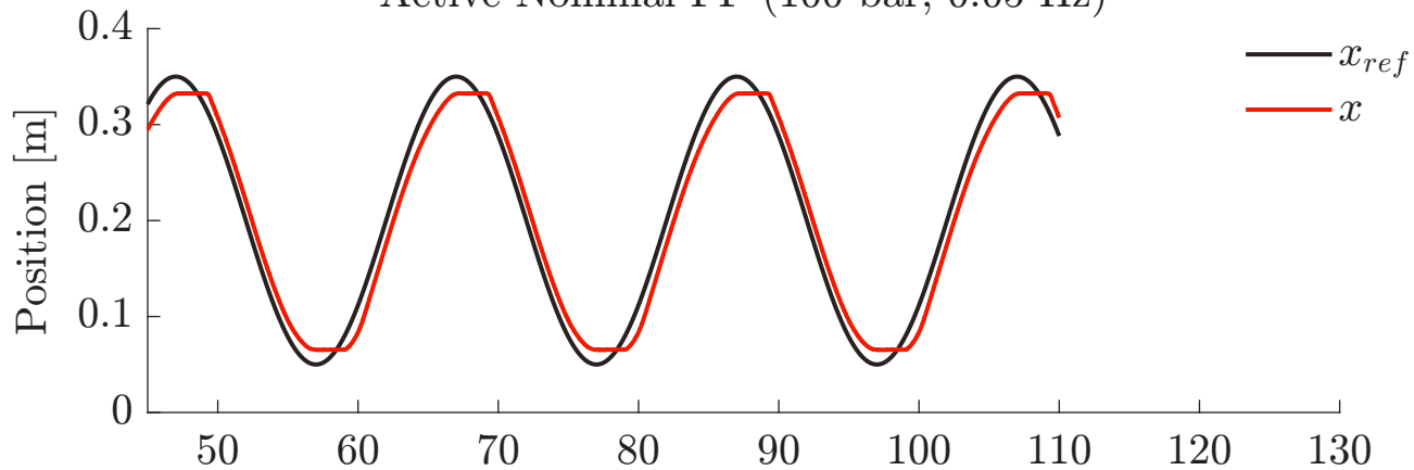
Active Nominal FF (100 bar, 0.05 Hz)
