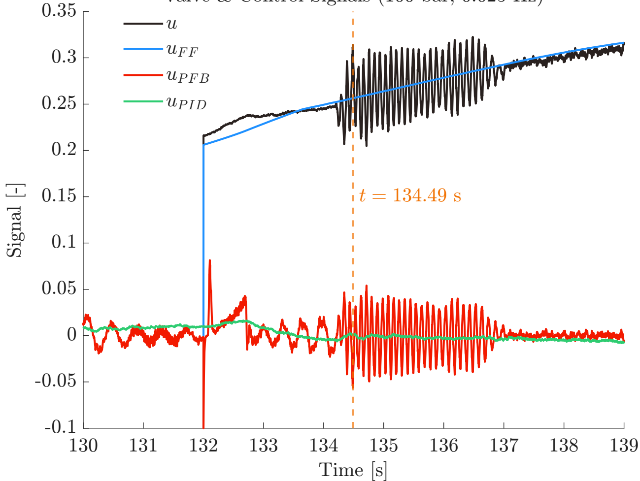
Valve & Control Signals (100 bar, 0.025 Hz)
