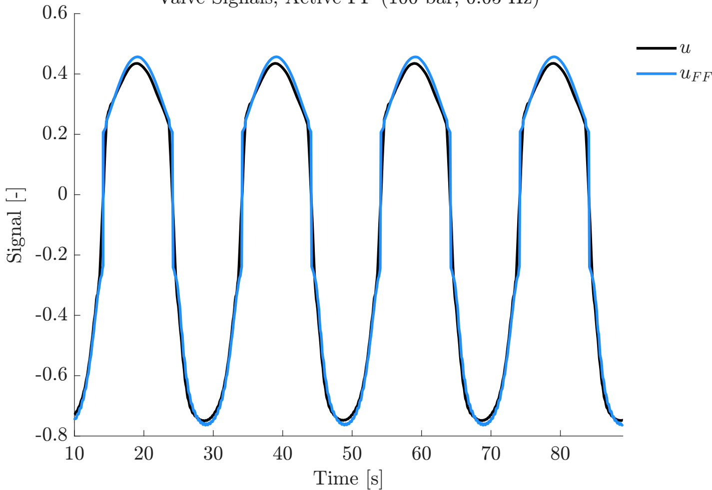
Valve Signals, Active FF (100 bar, 0.05 Hz)
