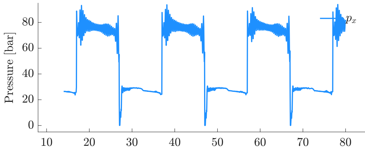
Pressure Feedback (100 bar, 0.05 Hz) - Selected Pressure
