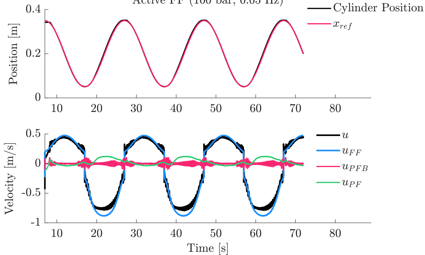
Active FF (100 bar, 0.05 Hz)
