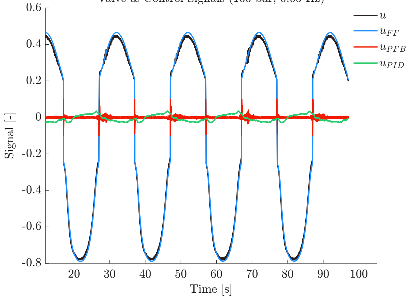
Valve & Control Signals (100 bar, 0.05 Hz)
