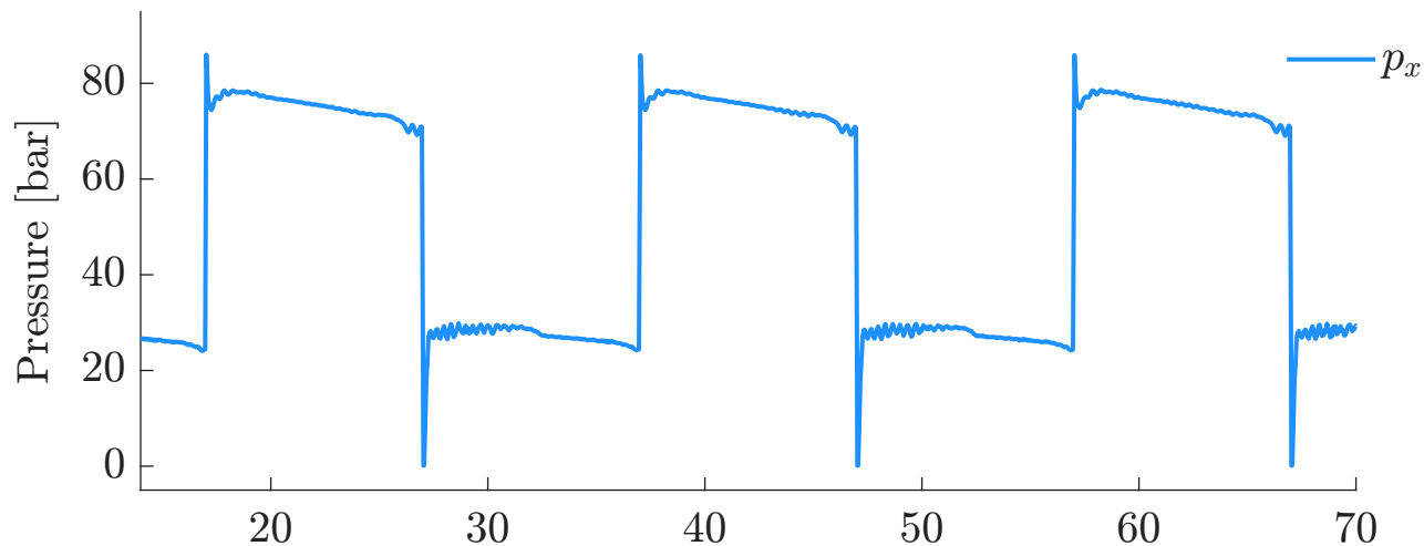
Pressure Feedback (100 bar, 0.05 Hz) - Selected Pressure
