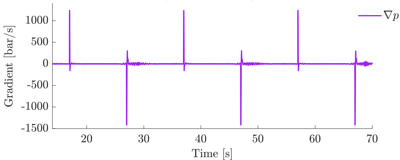
Pressure Feedback (100 bar, 0.05 Hz) - Pressure Gradient
