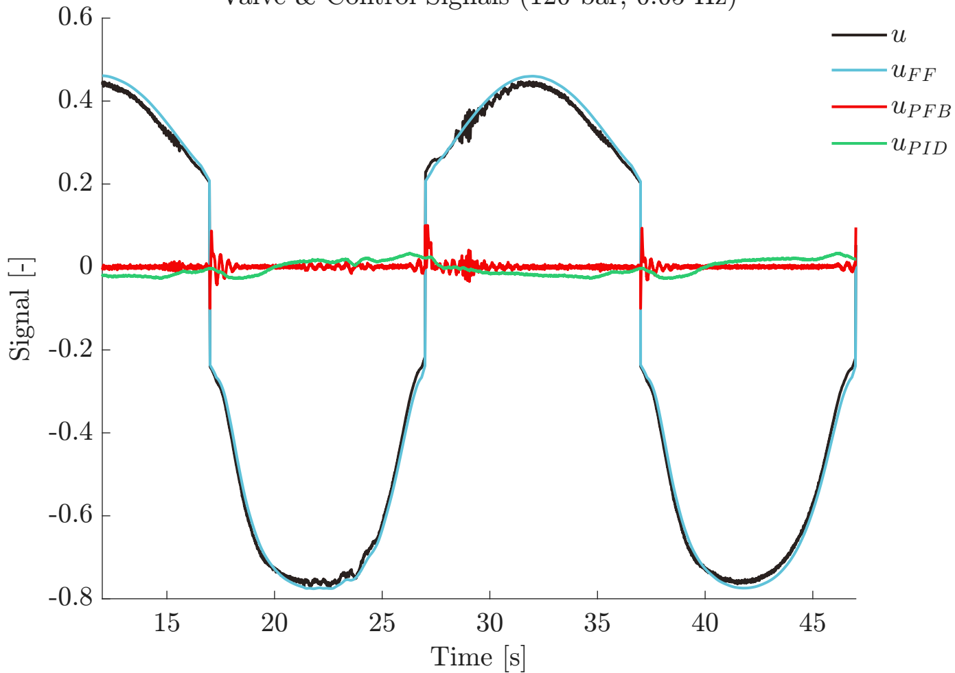
Valve & Control Signals (120 bar, 0.05 Hz)
