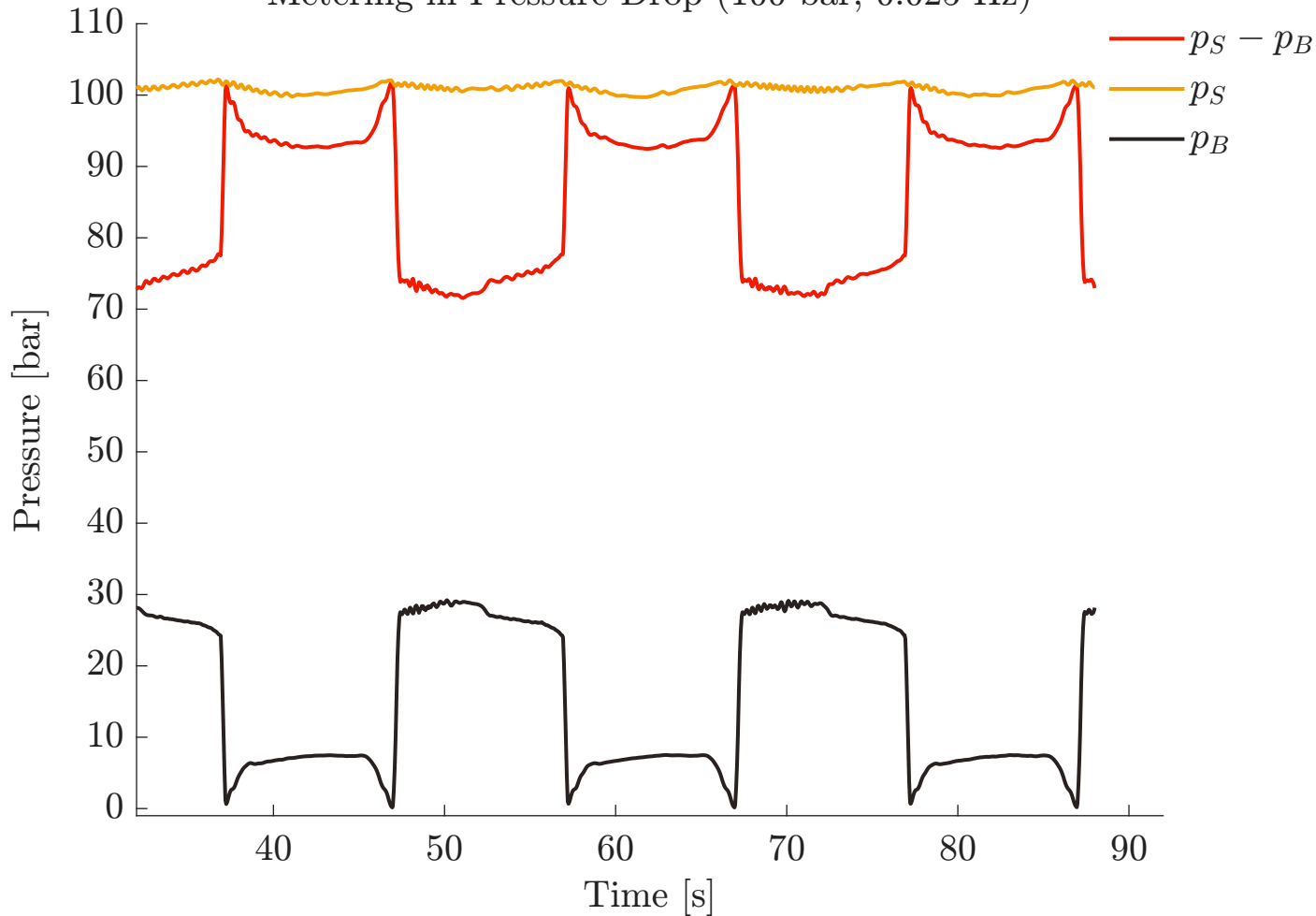
Metering-in Pressure Drop (100 bar, 0.025 Hz)
