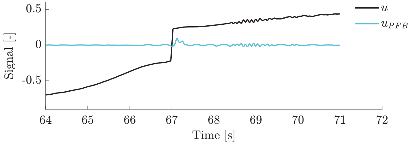
Pressure Feedback (100 bar, 0.05 Hz) - Valve Signals
