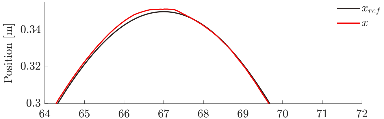
Pressure Feedback (100 bar, 0.05 Hz) - Cylinder Position
