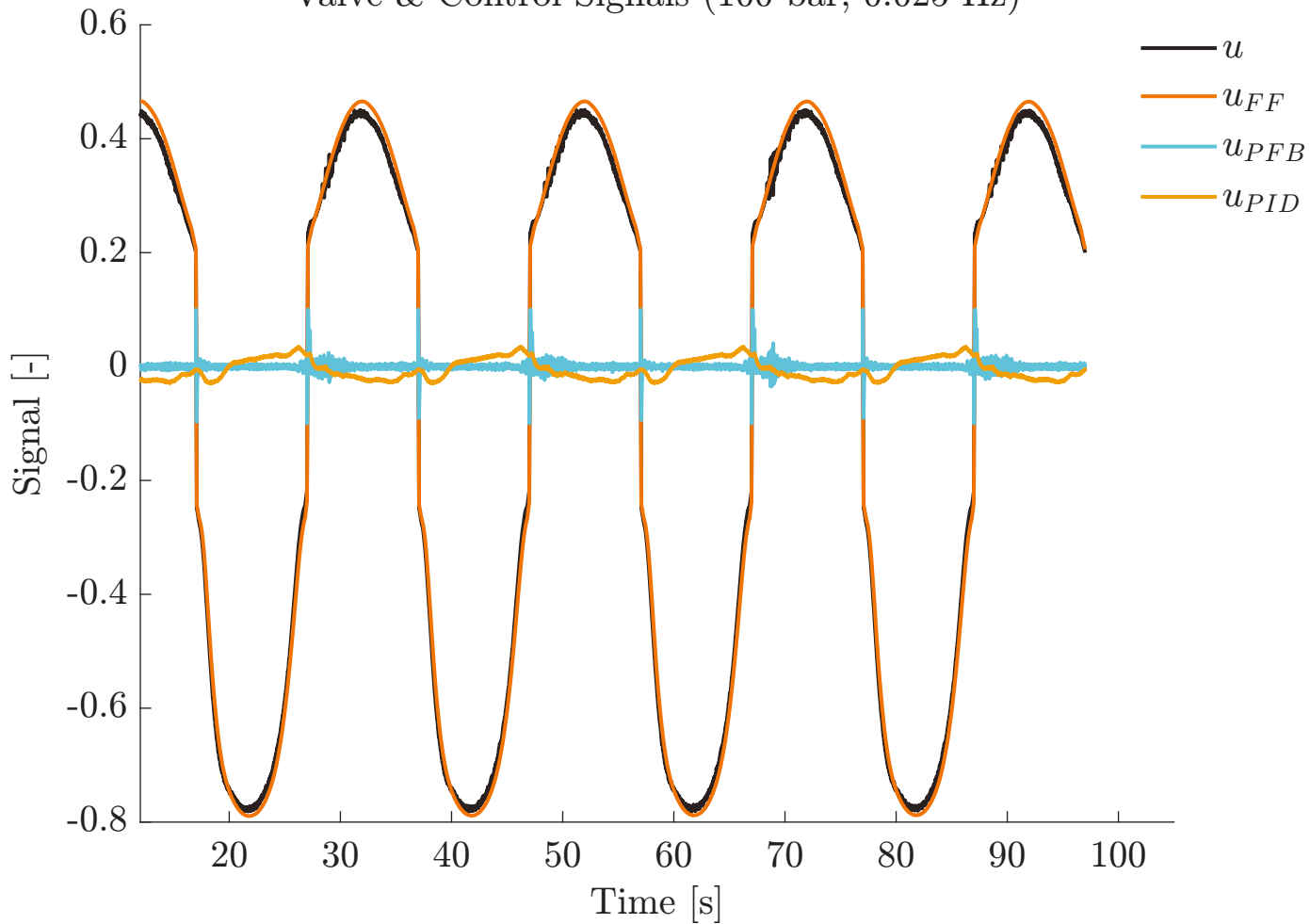
Valve & Control Signals (100 bar, 0.025 Hz)
