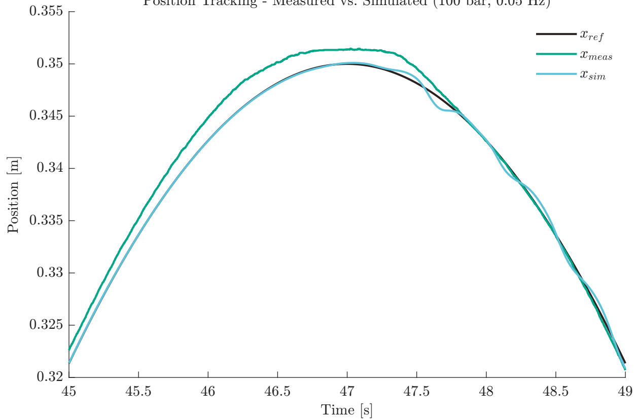
Position Tracking - Measured vs. Simulated (100 bar, 0.05 Hz)
