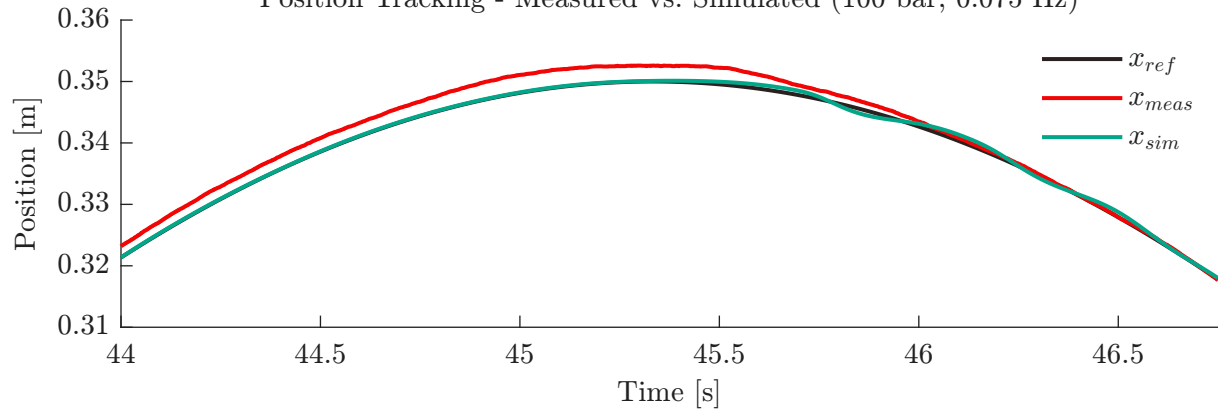
Position Tracking - Measured vs. Simulated (100 bar, 0.075 Hz)
