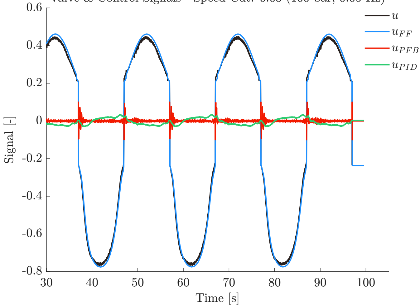
Valve & Control Signals - Speed Cut: 0.03 (100 bar, 0.05 Hz)
