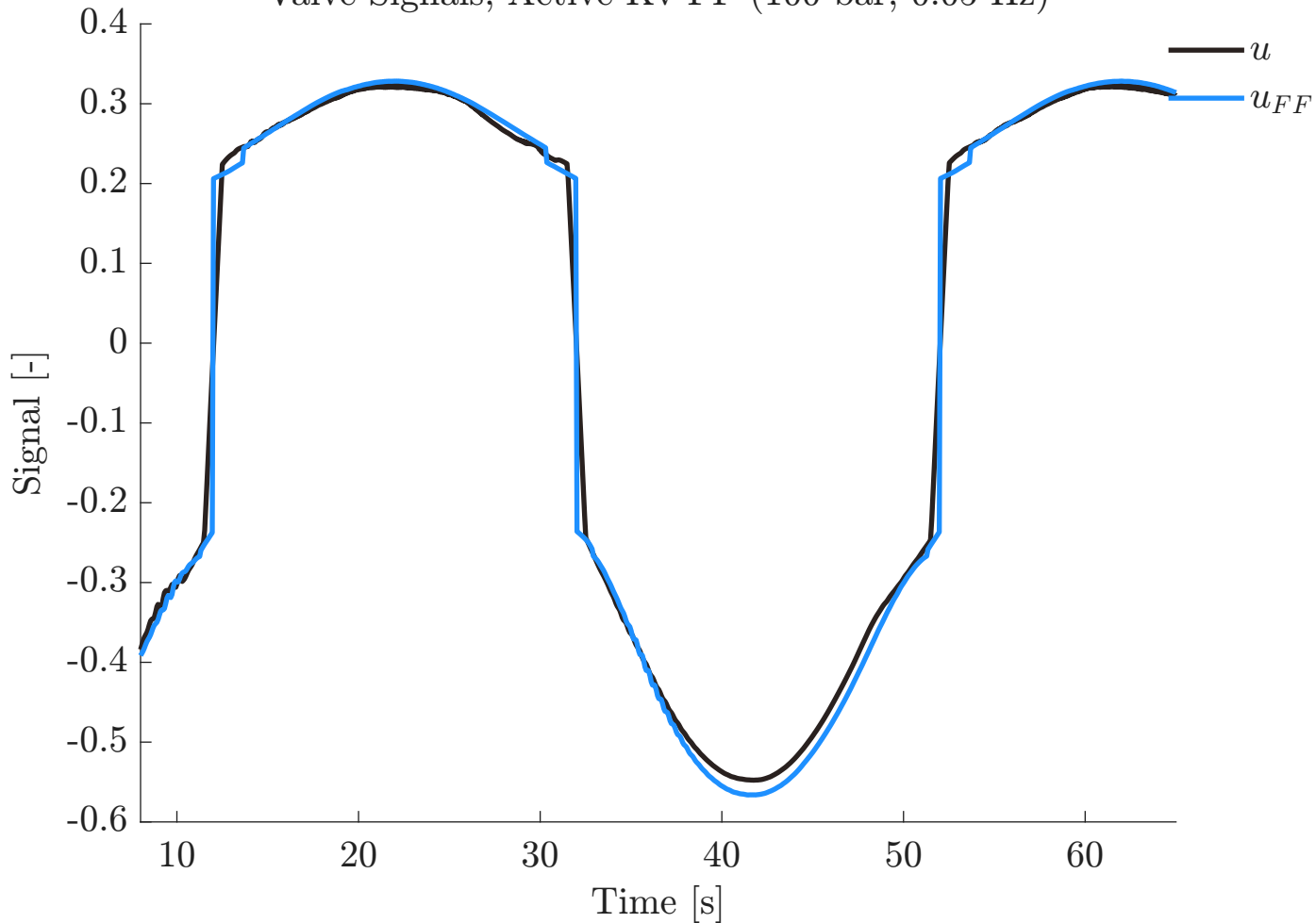
Valve Signals, Active Kv FF (100 bar, 0.05 Hz)
