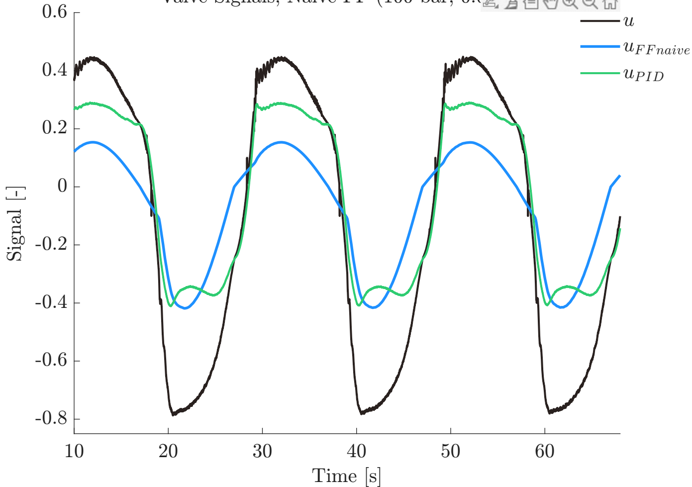
Valve Signals, Naive FF (100 bar, 0.0
