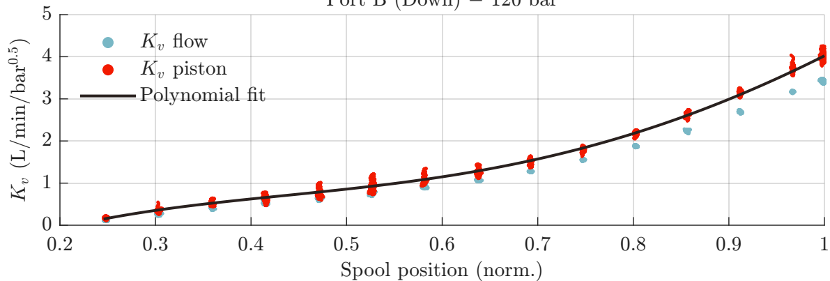
Port B (Down) – 120 bar
